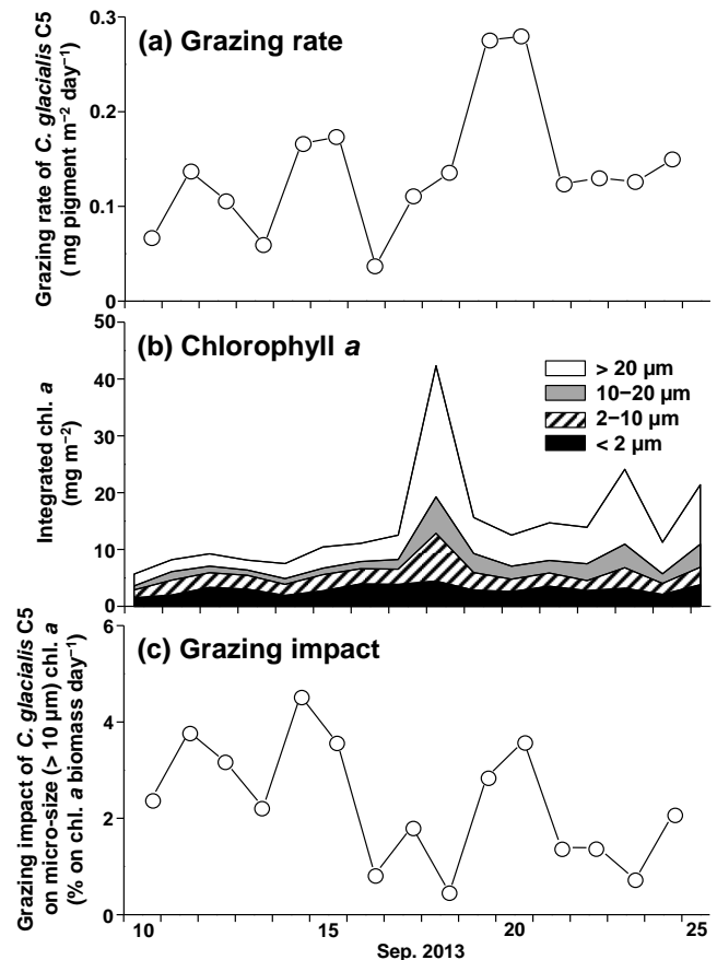
Figure 6. Temporal changes in the grazing rate of Calanus glacialis C5 (a), integrated size-fractionated chlorophyll a (b) and grazing impact of C. glacialis C5 on micro-phytoplankton (> 10 \mu\text{m} ) (c) at a fixed station in the Chukchi Sea from 10 to 25 September 2013.
