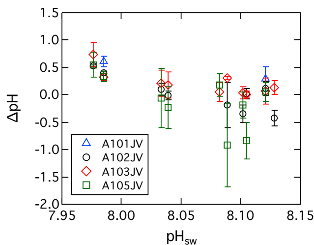
Figure 7. The calculated pH discrepancy ( \Delta\text{pH} = \text{pH}_{\text{shell}} - \text{pH}_{\text{sw}} ) shows a statistically significant negative relationship to \text{pH}_{\text{sw}} ( R^2 = 0.35 ; p value \leq 0.001 ). The negative correlation supports the argument that A. islandica regulate their EPF pH for calcification. The shell calcification pH ( \text{pH}_{\text{shell}} ) were calculated based on in situ water temperature \alpha = 1.0272 (Klochko et al., 2006).
