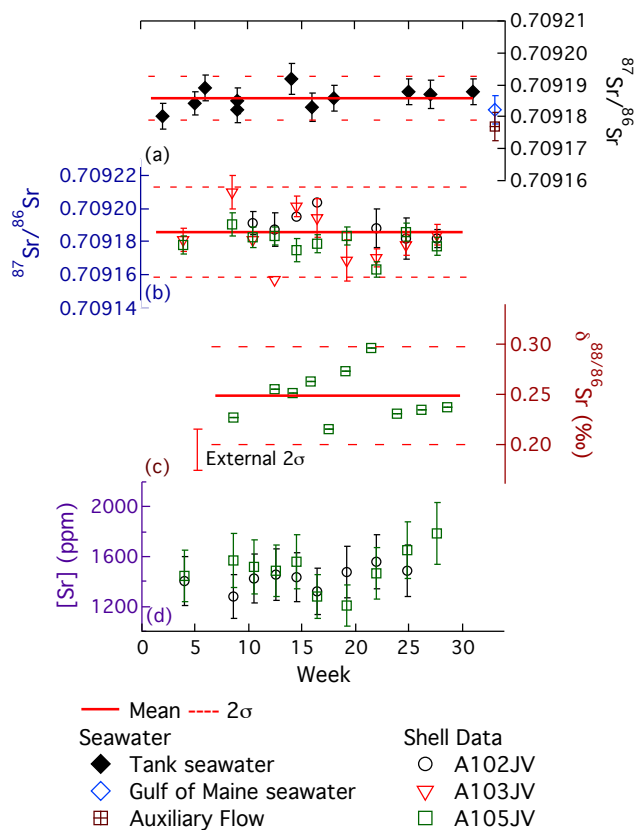
Figure 5. GoM ^{87}\text{Sr}/^{86}\text{Sr} data for (a) seawater samples and (b) shell samples, and the double-spike deconvolved (c) \delta^{88/86}\text{Sr} values and (d) Sr concentrations for the juvenile shell.
