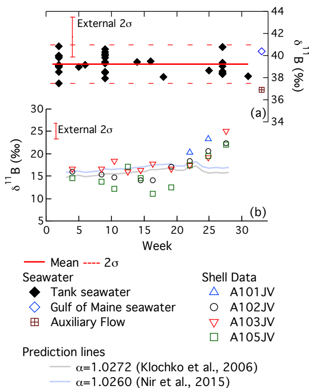
Figure 6. GoM boron data for (a) seawater samples and (b) shell samples. Two prediction lines listed were calculated based on our instrumental culture seawater pH, temperature, and salinity data, and two boron fractionation factors: \alpha = 1.0272 (Klochko et al., 2006) and \alpha = 1.0260 (Nir et al., 2015), where \alpha \equiv \frac{(^{11}\text{B}/^{10}\text{B})_{\text{B(OH)}_3}}{(^{11}\text{B}/^{10}\text{B})_{\text{B(OH)}_4^-}} . Equation (4) was used for the calculation.
