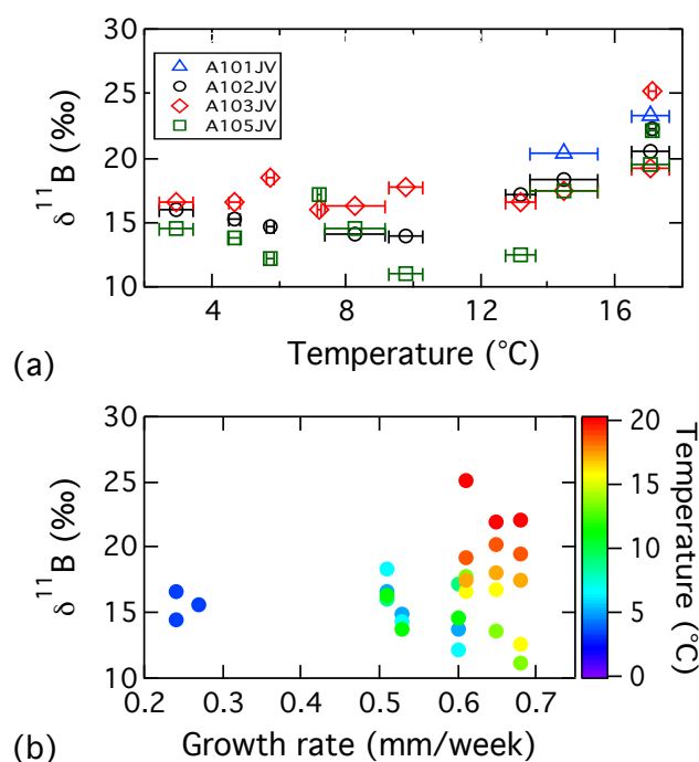
Figure 8. The comparisons between the shell \delta^{11}\text{B} and (a) the corresponding culture water temperature and (b) the growth rates for individual shells. Colors shown in (b) represent the temperature corresponding to each data point, with low temperatures in blue to high temperatures in red.
