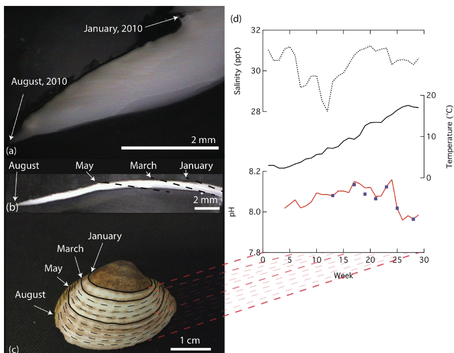
Figure 1. Photos of (a) adult and (b, c) juvenile A. islandica from the culture experiment. External marks on the shell or calcein marks in the cross section were used to constrain shell growth. (d) shows the corresponding in situ measurements of tank water salinity, temperature and pH during the 31-week culture experiment. The juvenile shells were sampled in 10 intervals for this study (c). Note that because the growth rates differ during the season, each interval represents different time durations (c, d).
