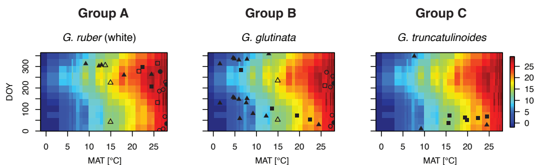
Figure 7. As Fig. 5, but peak timing patterns plotted over contour plots of annual temperature cycle. See Fig. S8 for other species. Symbols denote ocean basins: squares represent the Atlantic Ocean, circles the Indian Ocean and triangles the Pacific Ocean. Open symbols indicate sites affected by upwelling.
