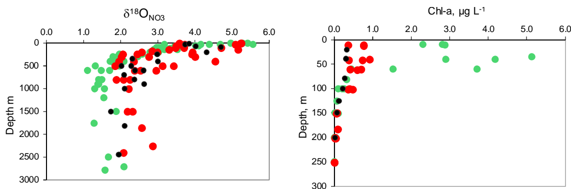
Figure 5. Profiles of \delta^{18}\text{O}_{\text{NO}_3} and \text{Chl a} ( \mu\text{g L}^{-1} ) profile for stations underlying the high chlorophyll plume in the vicinity of the Polar Front (green circles; stations TEW-7, TEW-8, F-L) and in the central part of the Polar Front Meander (red circles; stations TNS-6, TNS-1, TEW-6) and the reference station (black circles; station R-2).
