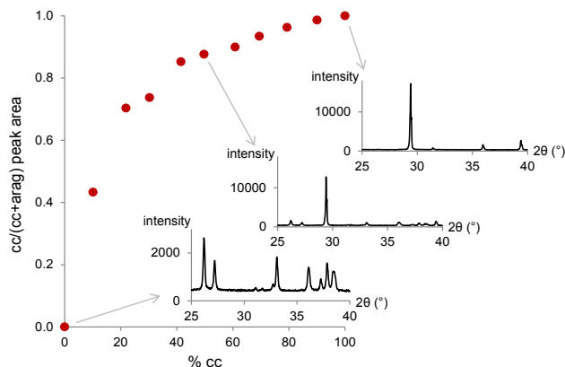
Figure 1. Standard calibration curve for quantifying the proportions of calcite and aragonite using XRD. Analyses used a \text{Cu-K}\alpha X-ray source (40 mA and 40 kV) with the sample loaded on a fixed stage while 2\theta varied through 25\text{--}40^\circ with a 0.004^\circ step size ( 0.05^\circ\text{s}^{-1} ). Areas under the calcite (cc) peak at 29.4^\circ and the aragonite (arag) peak at 26.2^\circ were used to calculate the proportional intensity of calcite as \text{cc}/(\text{cc} + \text{arag}) . Insets show standard intensity vs. 2\theta -angle XRD spectra for 0 % (pure aragonite), 49.7 %, and 100 % calcite (note the relative change in the vertical axis for the 0 % calcite/pure aragonite standard).
