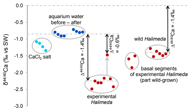
Figure 4. Ca-isotope data from the Halimeda experiment as well as wild Halimeda measured in this study. Note that \Delta^{44/40}\text{Ca} values, the offsets between growth medium and skeleton, are similar for the majority of the experimental and wild Halimeda , despite different \delta^{44/40}\text{Ca} values.
