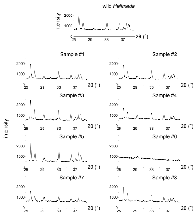
Figure 2. XRD spectra of the experimental Halimeda and a wild specimen. Note the small calcite peak and lack of aragonite peaks present for sample #6.
