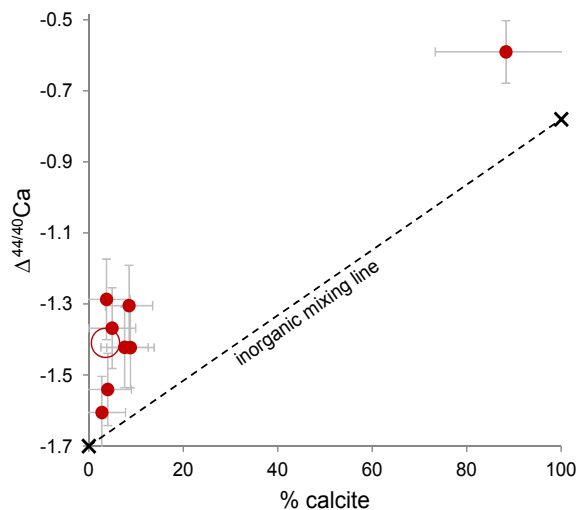
Figure 5. Ca-isotope ratios for Halimeda grown in experimental Cretaceous seawater, plotted against the percentage of calcite determined by XRD analysis. The open circle represents the average value for natural, ocean-grown Halimeda . The black line represents a mixing relationship between the inorganic calcite and aragonite endmembers from Marriott et al. (2004) and Gussone et al. (2005), respectively, at 15 °C. The Halimeda data occupy a region of similar slopes and approximately 0.25 ‰ heavier values than inorganic carbonate.
