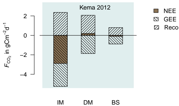
Figure 5. Simulated carbon fluxes at Kema in 2012 (46 days: 12 July to 26 August 2012) for IM, DM, and BS. Hatched bars denote the simulated GEE and R_{eco} , the sum is the NEE (brown bar).
