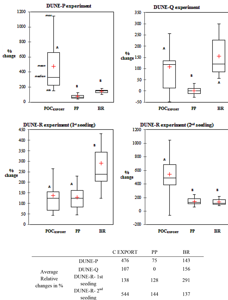
Figure 2. Box plots of the net fluxes expressed in relative change (%) and table with the average relative changes after the DUNE-P, -Q, -R1 and -R2 seedings, in percentage. The letters indicate the results of the statistical test in between the percentage of change for the \text{POC}_{\text{export}} , PP and BR. Means that were not significantly different between the different parameters ( p > 0.05 ) were labeled with the same letter. The mean relative changes (RC, in %) = (X_{\text{Dust}} - X_{\text{Control}}) \times 100 / X_{\text{Control}} with X_{\text{Control}} is the mean for the three mesocosms CONTROL.
