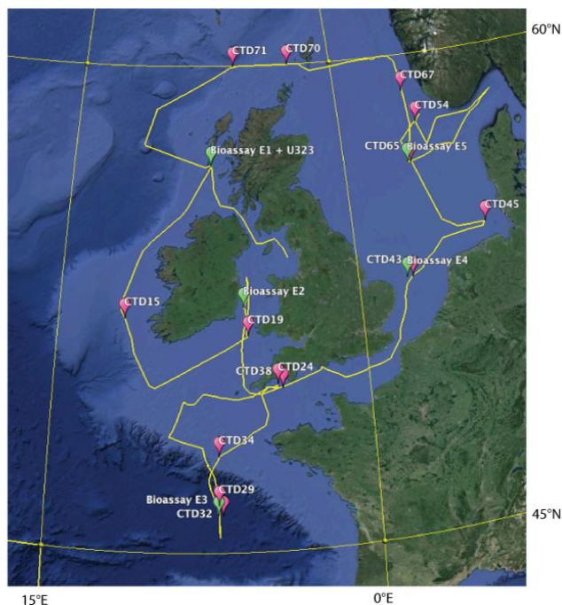
Figure 1. Track of cruise D366 and location of samples studied in detail here. Cartography, Google Earth.
