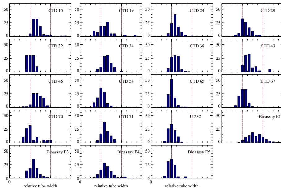
Figure 7. Frequency histograms of relative tube width in near-surface samples from CTD casts and the bioassay initial samples. Vertical axis is percentage abundance, based on measurement of ca. 60 coccoliths per sample. Total variability is fairly low, heavily calcified coccoliths (relative tube width > 0.4) are virtually absent, nonetheless there is still considerable variation in degree of calcification between samples.
