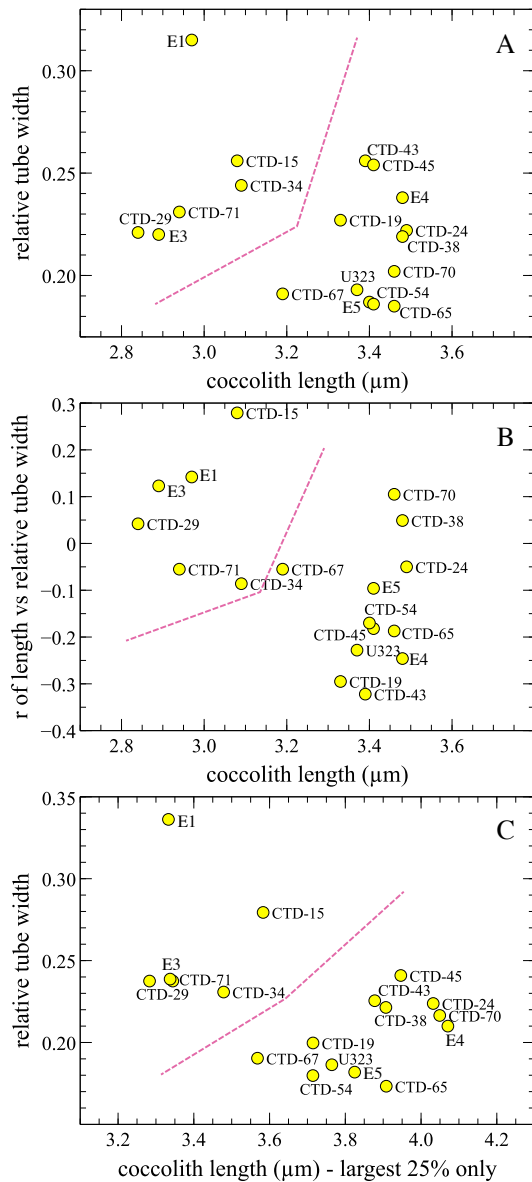
Figure 10. Relationship between relative tube width and coccolith length. (a) Relative tube width vs. coccolith length, the oceanic samples (to left of pink dotted line) are smaller but poorly separated on relative tube width. (b) Correlation coefficient of relative tube width vs. coccolith length. (c) Mean coccolith length vs. relative tube width for the largest 25 % of the coccoliths per sample, showing consistent separation of the samples into two sets, corresponding to oceanic vs. neritic locations.
