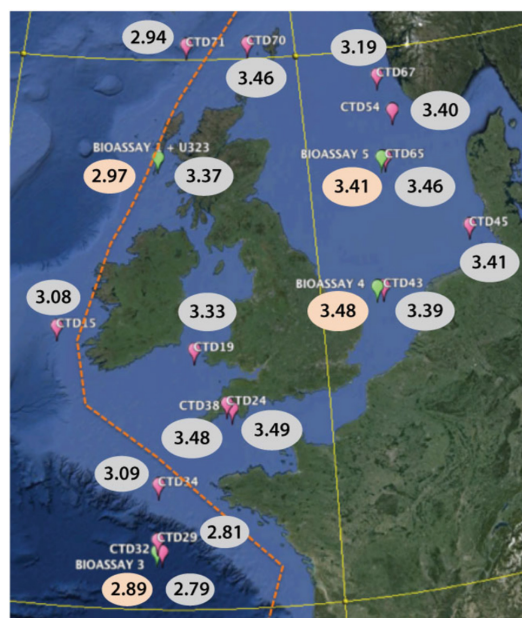
(a) mean coccolith lengths ( \mu\text{m} )
