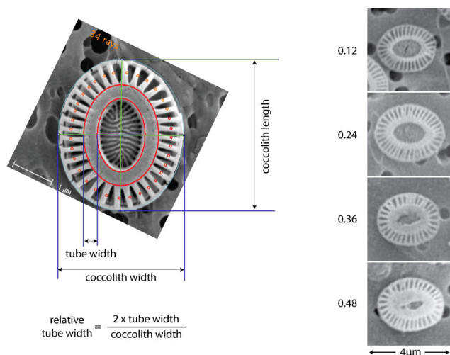
Figure 2. Morphometric parameters measured. Scanning electron micrograph (SEM) of an Emiliana huxleyi coccolith in distal view. Right hand panel – four E. huxleyi type A coccolith specimens from this study illustrating variation in relative tube width from 0.12 to 0.48 – this parameter is used here as an index of calcification.
