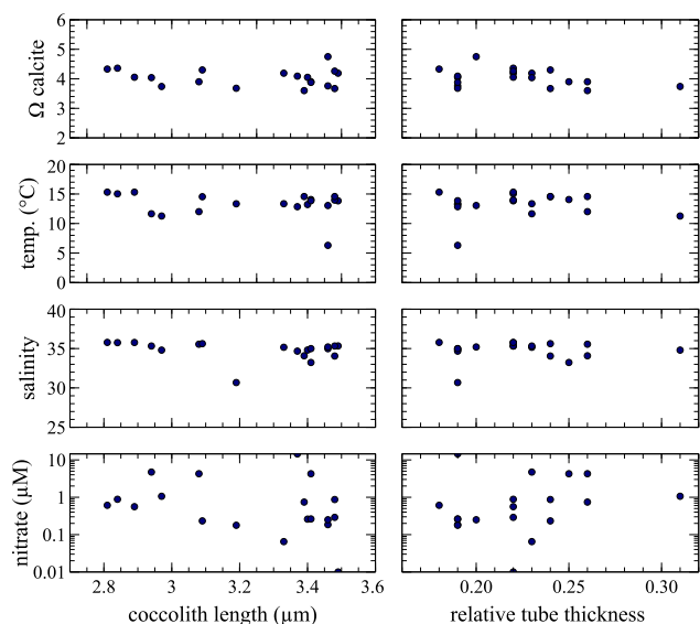
Figure 8. Mean values per sample of coccolith length and relative tube thickness from the 19 CTD and bioassay initial samples, as per the histogram of Figs. 6 and 7, plotted against carbonate chemistry, temperature, salinity and nutrient concentration. Nitrate and phosphate concentrations are strongly correlated in the sample sets ( R = 0.96 ) so only nitrate (strictly nitrate + nitrite) concentration is plotted, this is shown on a logarithmic axis owing to high variability in absolute values. There is no obvious relationship of the morphological parameters to any of the environmental parameters, and correlation coefficients were below significance levels.
