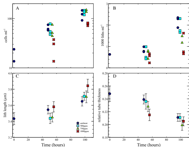
Figure 4. Enlarged plots of Emiliania huxleyi abundances (a, b) and morphometrics (c, d) from Bioassay E4, with vertical axes adjusted to emphasise the data. Symbols indicate the culture conditions. Plot (a) of cell abundance is on a logarithmic scale. On plots (c) and (d) the vertical bars are standard errors of the mean, (standard deviation over square root of the sample number), which provides an estimate of possible error in the mean value.
