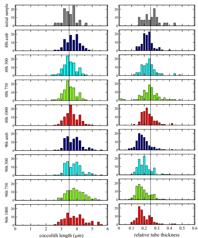
Figure 5. Raw morphometric data from Bioassay E4 plotted as frequency histograms. Vertical scale is percentage abundance. Colour coding is the same as for the symbols on Figs. 3 and 4. Vertical lines through the data sets represent the mean values in the initial sample; by the end of the experiment (96 h) coccolith length had increased significantly and relative tube width decreased significantly but with very little variation between treatments.
