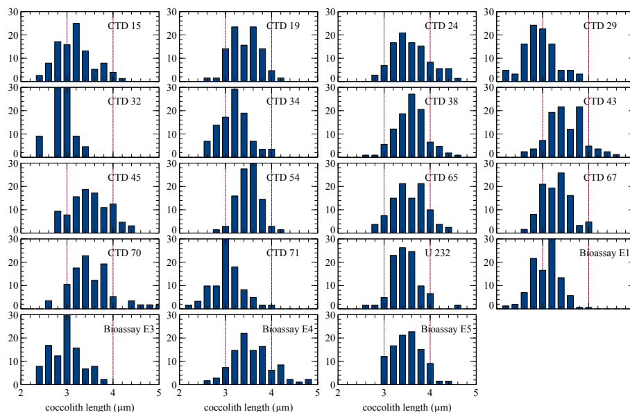
Figure 6. Frequency histograms of coccolith length from near-surface samples from CTD casts and the bioassay initial samples. Vertical axis is percentage abundance, based on measurement of ca. 60 coccoliths per sample. There is clearly significant inter-sample variability between locations.
