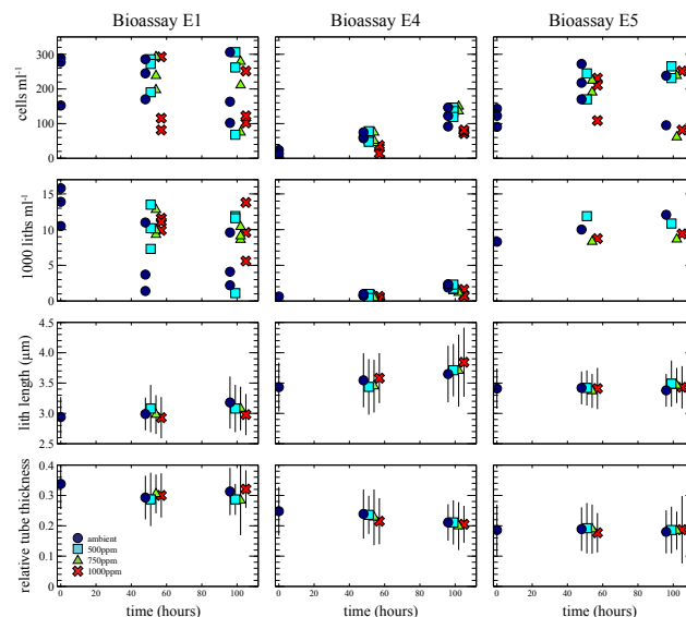
Figure 3. Emiliana huxleyi abundances and morphometrics from bioassays E1, E4 and E5. Top two rows of panels cell abundance and loose coccolith abundance over time. Symbols indicate the culture conditions. There are usually three replicates per time point and culture condition. Sampling was carried out at 48 and 96 h but samples from separate conditions are moved slightly along the x axis. Lower two rows of panels coccolith length and relative tube thickness over time. Symbols indicate averages from ca. 60 measurements per sample and vertical bars indicate \pm 1 standard deviation.
