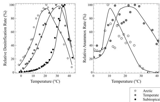
Fig. 5. Left: normalized temperature response of denitrification for subtropical, temperate, and Arctic sites. Right: normalized temperature response of anammox for temperate and Arctic sites. Curves were visually fit and error bars are omitted for clarity.
