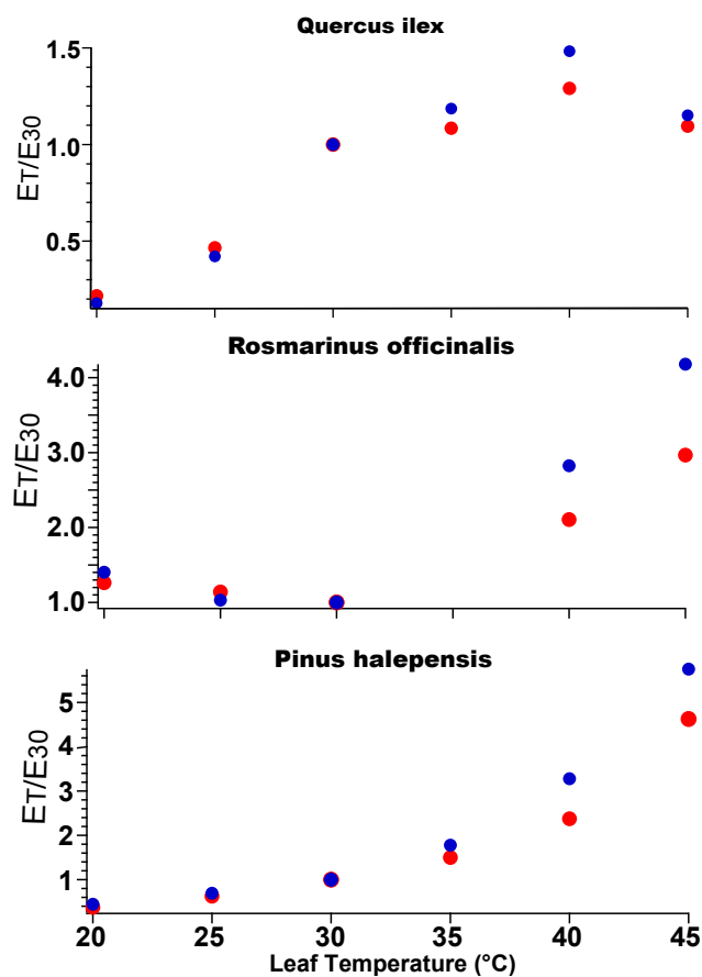
Fig. 6. An example of (-)/(+) - \alpha -pinene emission which was normalized by dividing by emission at 30 °C from different plant species in dependency with temperature. The red points represent normalized (-) - \alpha -pinene emissions and the blue points show the normalized (+) - \alpha -pinene emissions.
