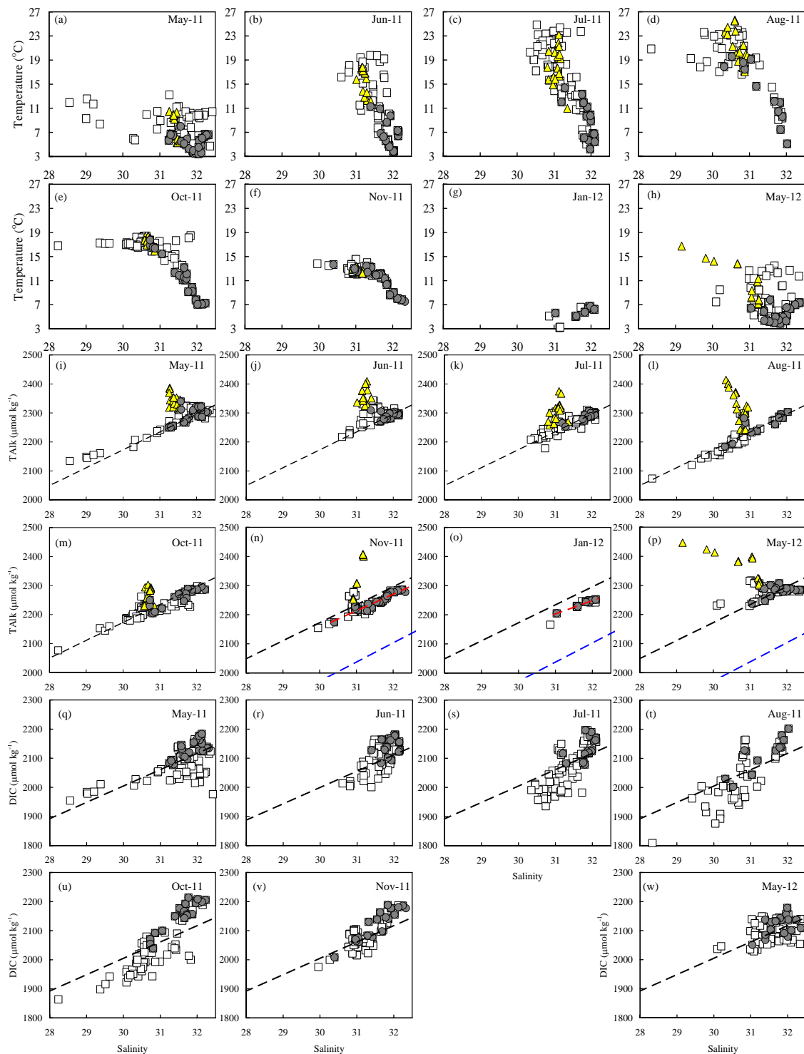
Fig. 6. Plots of temperature versus salinity (a–h), total alkalinity versus salinity (i–p), and dissolved inorganic carbon versus salinity (q–w) for each cruise. Open rectangles show all data in water columns in the study area, and grey circles represent bottom-water data in the study area. Yellow triangles denote the adjacent Bohai Sea data. Black dashed lines are \text{TALK} (\mu\text{mol kg}^{-1}) = 61.745 \times \text{Salinity} + 320 (i–p) and \text{DIC} (\mu\text{mol kg}^{-1}) = 56.161 \times \text{Salinity} + 320 (q–w), which are supposed as the bottom-water mixing lines from May to October. Red dashed lines in panels (n–o) are regression lines of total alkalinity in bottom waters, i.e. \text{TALK} (\mu\text{mol kg}^{-1}) = 56.814 \times \text{Salinity} + 452 in November, and \text{TALK} (\mu\text{mol kg}^{-1}) = 45.404 \times \text{Salinity} + 795 in January. Blue dashed lines in panels (n–p) are \text{TALK} (\mu\text{mol kg}^{-1}) = 2305/35 \times \text{Salinity} , which is the ideal mixing line between adjacent open ocean surface waters and rainwater (Chen and Wang, 1999; Lee et al., 2006).
