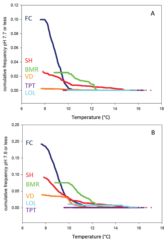
Fig. 2. Cumulative frequencies of exposure to pH (total scale) less than 7.7 (A) and 7.8 (B) as recorded at 10 min intervals by in situ Durafet ® -based pH sensors deployed in intertidal environment between April and September (maximum record length). Exposure frequencies at a given pH threshold are normalized to expanding windows of maximum to minimum in situ water temperature to illustrate the response of pH to the progressive strengthening of seasonal upwelling at each site.
