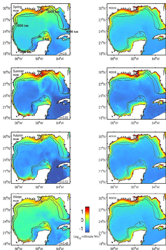
Fig. 8. Comparison of simulated (left panels) and MODIS observed (right panels) seasonal mean surface chlorophyll. Also shown in each panel are 50 (labeled with distance) and 200 m isobaths.
