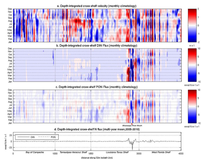
Fig. 12. Depth-integrated monthly mean cross-shelf (a) velocity, (b) DIN flux, (c) PON flux and (d) annual mean DIN and PON flux cross the 50 m isobath. Positive/negative values stand for shoreward/seaward transport.
