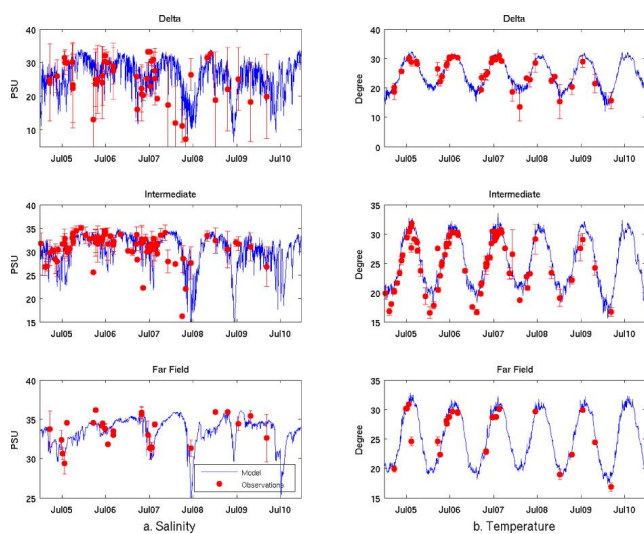
Fig. 6. Time series comparisons between observed and simulated (a) sea surface salinity (left panels) and (b) sea surface temperature (right panels) in 2005–2010. Results are presented for each of three subregions illustrated in Fig. 2. Blue lines are simulated values and filled red circles are observed values. Error bars stand for one standard deviation of available observations.
