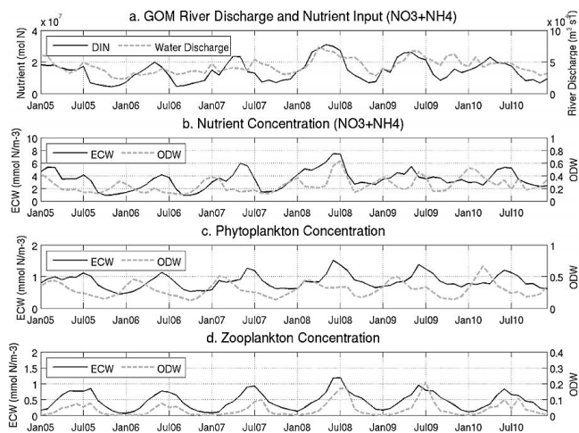
Fig. 10. Monthly mean time series of (a) river discharge and DIN loading, (b) surface DIN concentration, (c) surface phytoplankton concentration, and (d) surface zooplankton concentration on the shelf, and deep-sea areas over the entire gulf.
