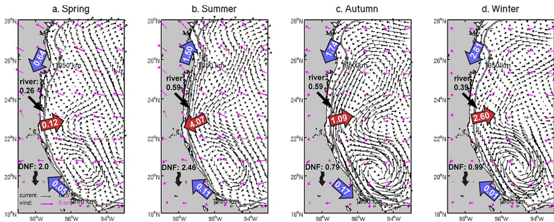
Fig. 14. Similar to Fig. 13 but for the TAVE shelf.
