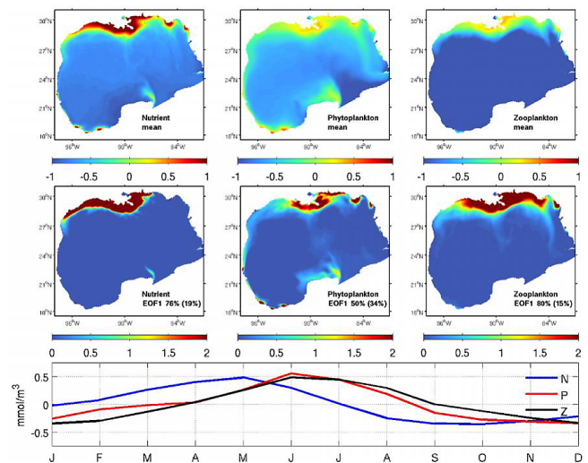
Fig. 11. EOF analyses of surface DIN, phytoplankton and zooplankton fields. Mean fields are shown in the top panels (units: \text{mmol N m}^{-3} , log scale), the first EOF modes and the variance they account for are shown in the middle panels and their corresponding first principle components are shown in the bottom panels.
