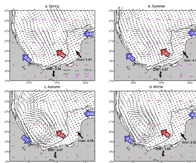
Fig. 13. Seasonal mean surface current and wind fields in the BOC shelf in (a) spring, (b) summer, (c) autumn, and (d) winter. Also shown is regional along-shelf nitrogen transport (blue arrows, unit: 10^9 \text{ mol N} ), cross-shelf nitrogen transport (red arrows, unit: 10^9 \text{ mol N} ), river inputs (unit: 10^9 \text{ mol N} ) and nitrogen removed by denitrification (DNF, unit: 10^9 \text{ mol N} ), and 50 m isobath (grey line).
