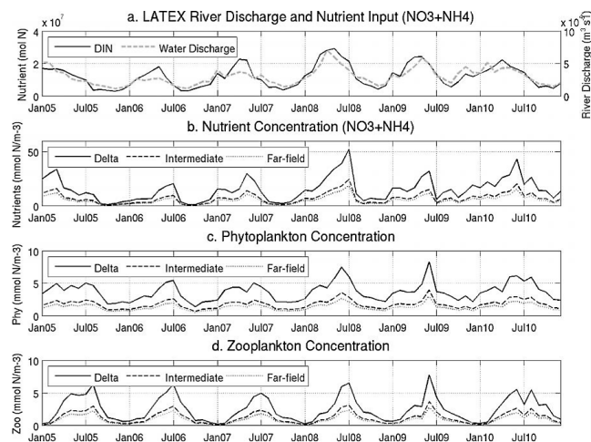
Fig. 9. Monthly mean time series of (a) river discharge and DIN loading, (b) surface DIN concentration, (c) surface phytoplankton concentration, and (d) surface zooplankton concentration in each of the three analysis regions (Delta, Intermediate, Far-field) on the LATEX shelf.
