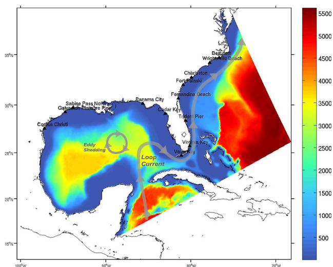
Fig. 1. The SABGOM ROMS model domain overlaid with water depth (color-shading), location of 13 tidal stations (black triangles), and a schematic circulation pattern.
