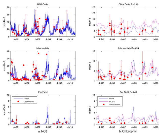
Fig. 7. Time series comparison between observed and simulated (similar to Fig. 6) (a) nitrate (left panel) and (b) chlorophyll (right panels). For chlorophyll comparison, MODIS monthly mean pigment concentration data (pink line) are also shown for each of three regions.
