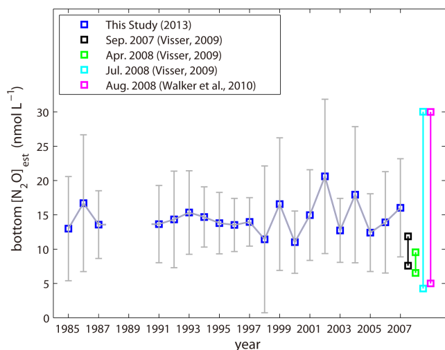
Fig. 2. Interannual variation of estimated bottom-water N 2 O concentrations (blue square) in the nGOM during July 1985–2007. Measurements are included (black, green, cyan, and pink squares: September 2007, April 2008, July 2008, and August 2008, respectively).
