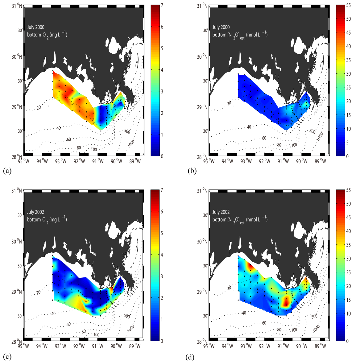
Fig. 5. Distributions of observed bottom-water O 2 and estimated bottom-water N 2 O concentrations in July 2000 and 2002, representing min. and max. hypoxic areal extent during the study period, respectively. (a) and (b) indicate bottom-water O 2 and N 2 O spatial distributions in July 2000. (c) and (d) denote bottom-water O 2 and N 2 O spatial distributions in July 2002.
