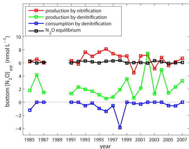
Fig. 3. The individual contributions of nitrification (red squares, production), denitrification (green squares, production), denitrification (blue squares, consumption), and N 2 O equilibrium (black squares) to the bottom-water N 2 O concentrations in the nGOM from July 1985 to 2007.
