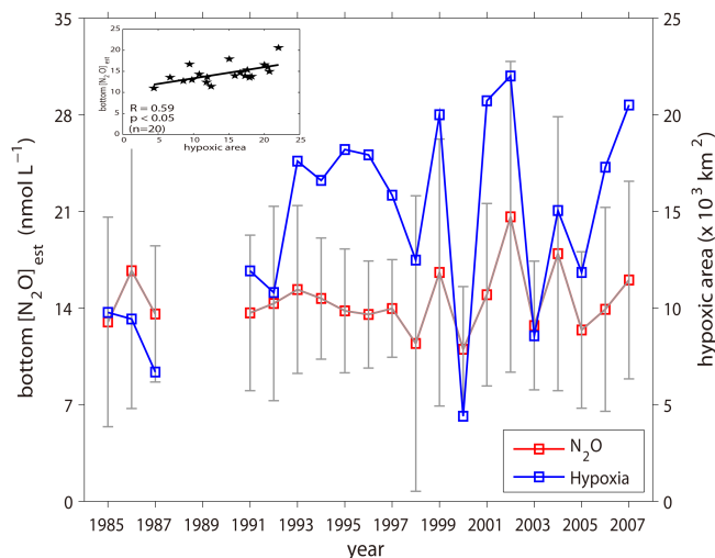
Fig. 4. Interannual variations in summer (July) bottom-water N 2 O concentration (nmol L -1 , red squares) and the areal extent of hypoxia (km 2 , blue squares). The estimated bottom-water N 2 O concentrations were significantly correlated with the areal extent of hypoxia ( R = 0.59 ; p < 0.05 with n = 20 ). Data concerning the areal extent of hypoxia are available at http://www.gulfhypoxia.net/Research/Shelfwide%20Cruises/ (data source: N. N. Rabalais, Louisiana Universities Marine Consortium, R. E. Turner, Louisiana State University).
