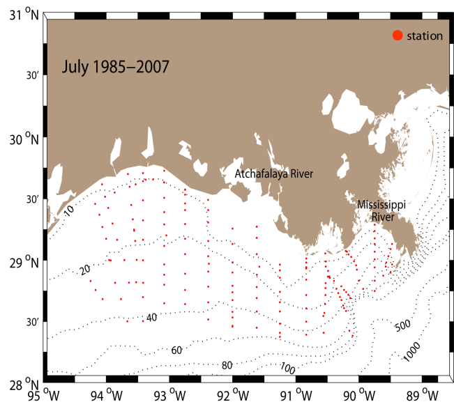
Fig. 1. The study area map showing the summer Texas–Louisiana shelf-wide cruise stations (red dots) during July 1985–2007 with the bathymetry contours (black dotted lines) in the northern Gulf of Mexico.
