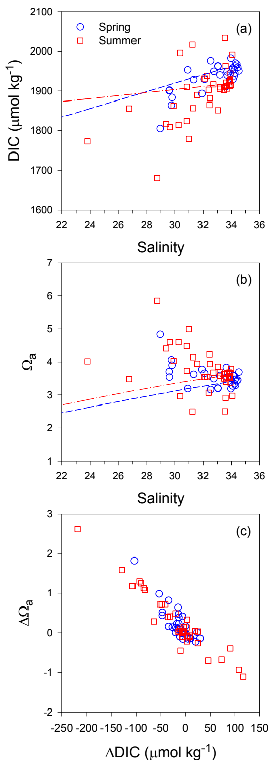
Fig. 7. Plots of (a) DIC vs. salinity, (b) \Omega_a vs. salinity, and (c) \Delta\Omega_a vs. \Delta\text{DIC} for the surface waters in the East China Sea in spring and summer 2009. The superimposed lines represent the hypothetical conservative mixing lines between the freshwater and seawater end-members. \Delta\Omega_a and \Delta\text{DIC} denote the difference between the measured values and the hypothetical conservative-mixing values.
