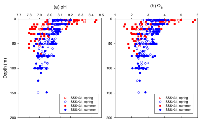
Fig. 10. Depth profiles of (a) pH 25 and (b) Ω a over the East China Sea shelf in spring and summer 2009. Squares and circles denote the data in (SSS < 31) and out (SSS > 31) of the Changjiang plume area, respectively. SSS: sea surface salinity.
