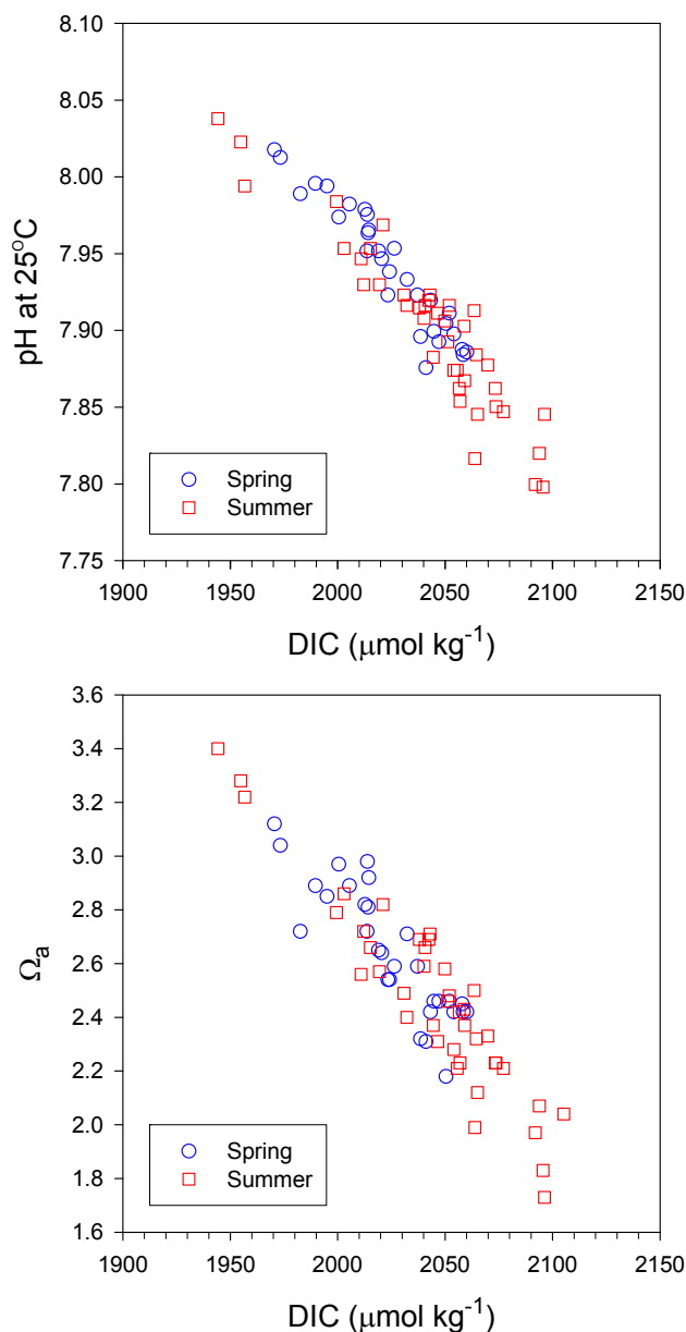
Fig. 11. Plots of (a) pH 25 vs. DIC and (b) Ω a vs. DIC for the bottom waters in the East China Sea during spring and summer 2009.
