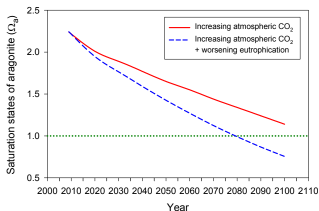
Fig. 12. The predicted time course of \Omega_a changes in the bottom water of the Changjiang plume area within the 21st century due to (i) atmospheric \text{CO}_2 increase (IPCC IS92a scenario; solid line), and (ii) the combined effect of atmospheric \text{CO}_2 increase and worsening eutrophication (dashed line).
