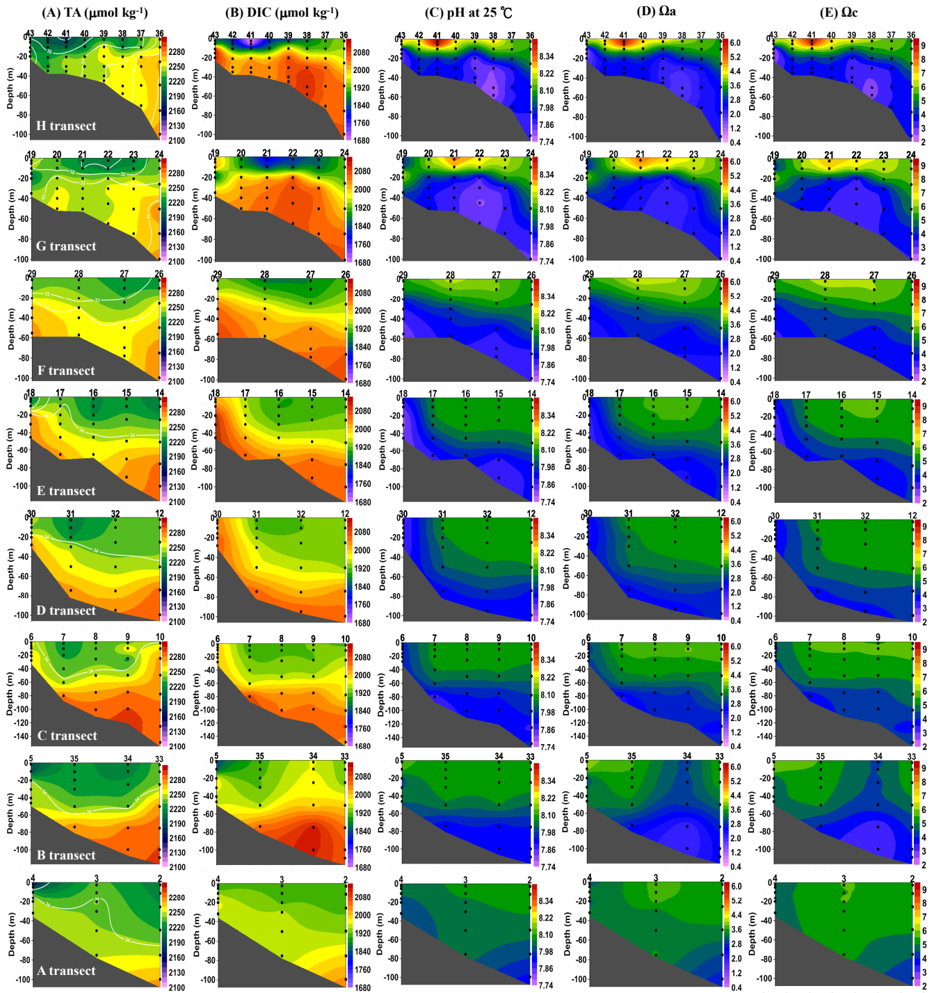
Fig. 5. Vertical distributions of TA, DIC, pH_{25} , \Omega_c and \Omega_a along the A to H transects in the East China Sea in summer 2009. Superimposed white lines on TA distributions are isohalines.
