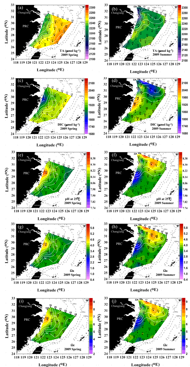
Fig. 3. Surface distributions of (a) TA in spring, (b) TA in summer, (c) DIC in spring, (d) DIC in summer, (e) pH_{25} in spring, (f) pH_{25} in summer, (g) \Omega_a in spring, (h) \Omega_a in summer, (i) \Omega_c in spring, and (j) \Omega_c in summer 2009 in the East China Sea. Superimposed white lines are isohalines.
