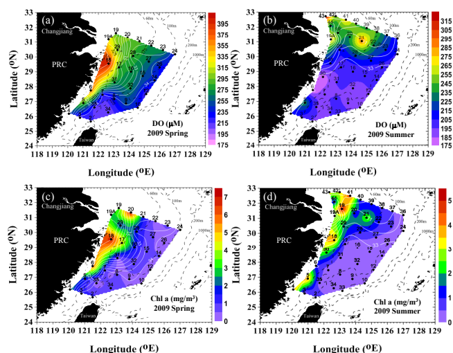
Fig. 6. Surface distributions of (a) dissolved oxygen (DO) in spring, (b) DO in summer, (c) Chl a in spring, and (d) Chl a in summer 2009 in the East China Sea. Superimposed white lines are isohalines.
