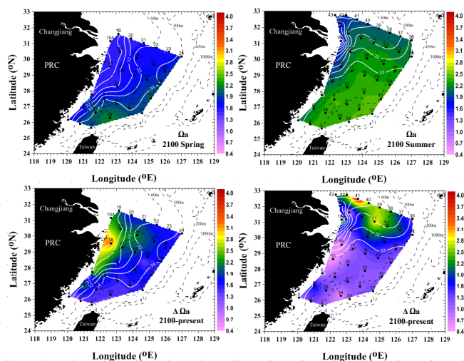
Fig. 8. (a) and (b) show predicted surface water \Omega_a on the East China Sea shelf in spring and summer by the year 2100, respectively. (c) and (d) show the difference of \Omega_a between the predicted \Omega_a in 2100 and its present value ( \Delta\Omega_a ) in spring and summer, respectively. Superimposed white lines are isohalines.
