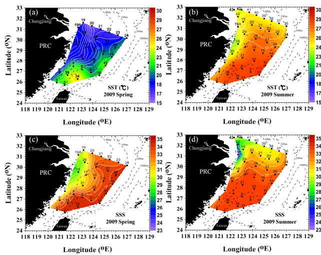
Fig. 2. Surface distributions of temperature (SST) are indicated in (a) and (b); and (c) and (d) indicate salinity (SSS) in spring (a and c) and summer (b and d) 2009 in the East China Sea.
