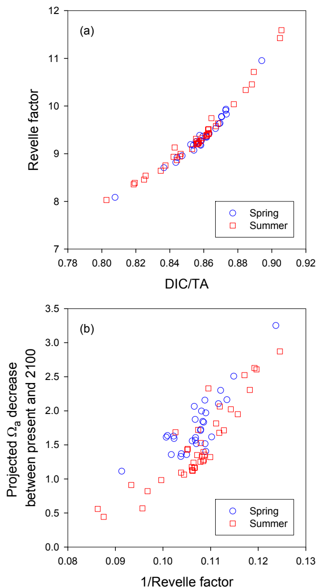
Fig. 9. Plots of (a) Revelle factor vs. DIC/TA ratio, and (b) difference of \Omega_a between the predicted \Omega_a in 2100 and its present value ( \Delta\Omega_a ) vs. the reciprocal of the Revelle factor ( 1/\text{Revelle factor} ) for the surface waters in the East China Sea during spring and summer 2009.
