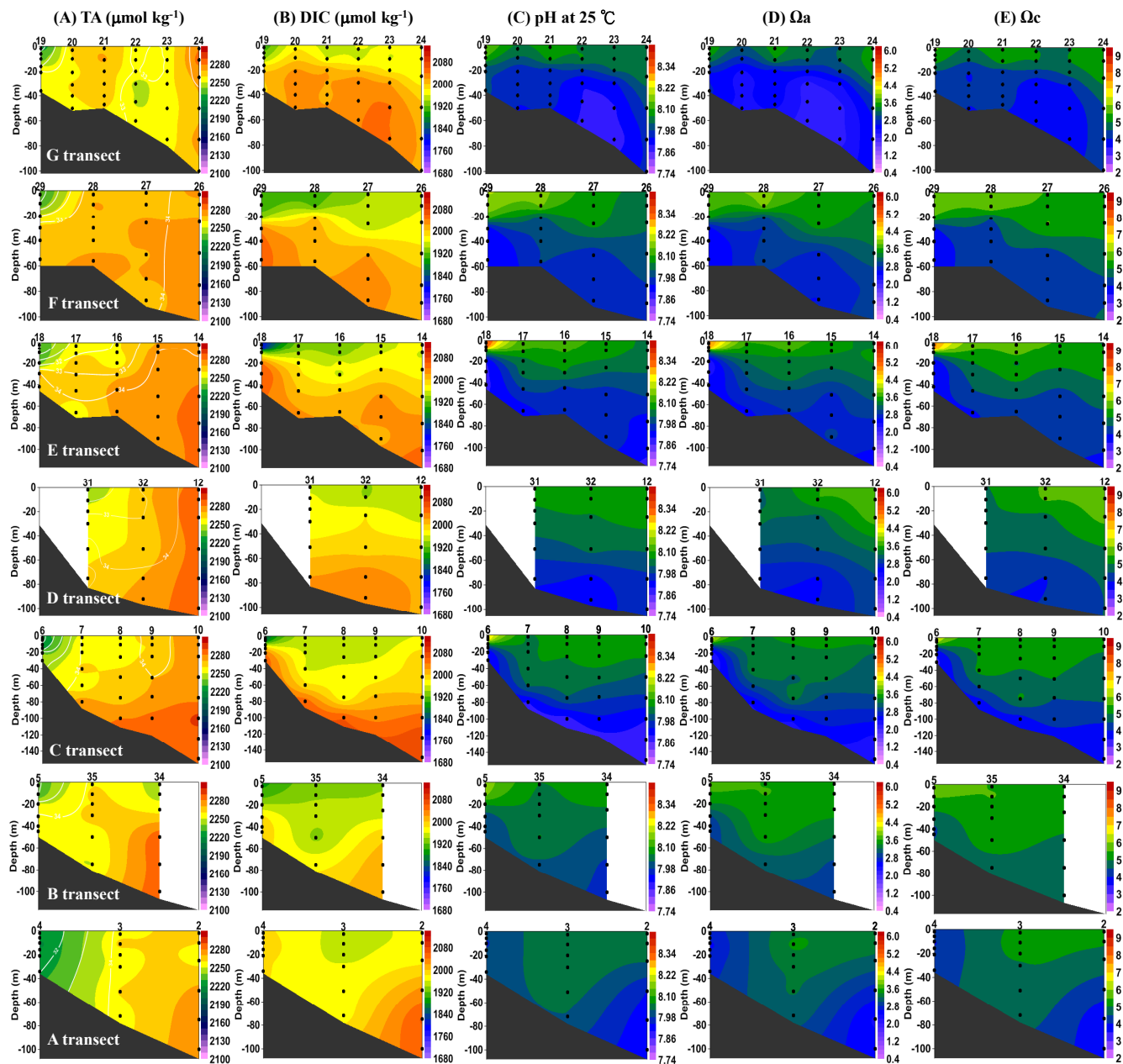
Fig. 4. Vertical distributions of TA, DIC, pH at 25°C, \Omega_c and \Omega_a along the A to G transects in the East China Sea in spring 2009. Superimposed white lines on TA distributions are isohalines.
