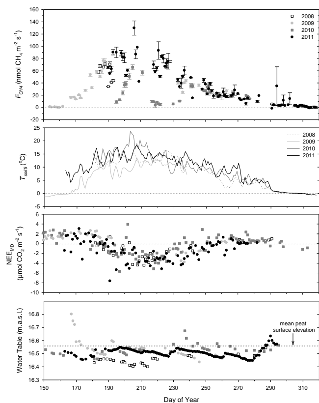
Fig. 2. Mean daily F_{\text{CH}_4} (no gap-filling) for 30 min averaged campaign periods ( n=1 to 48) \pm 1 SE (standard error) shown, and mean daily T_{\text{soil}5} , \text{NEE}_{\text{MD}} and water table height for all shoulder + growing seasons (DOY 150–320, 2008–2011).
