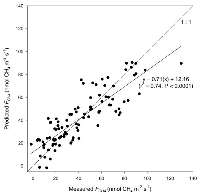
Fig. 6. Stepwise multiple linear model estimates of daily mean F_{\text{CH}_4} in relation to daily mean measured values for all measurement periods and years when water table height was below 16.61 m a.s.l. The model is F_{\text{CH}_4} = (-9.8 \times T_{\text{hol60}}) + (279.8 \times \text{water table}) + (1.7 \times T_{\text{air}}) - 4572.2 .
