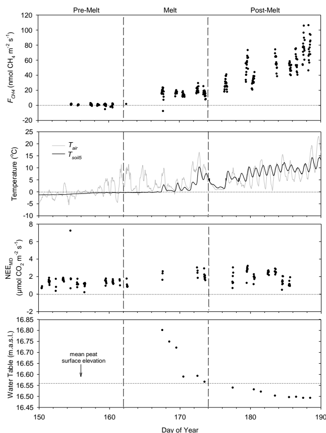
Fig. 1. Spring of 2009 30 min \text{CH}_4 flux ( F_{\text{CH}_4} ), air temperature ( T_{\text{air}} ), 5 cm soil temperature ( T_{\text{soil5}} ), midday net \text{CO}_2 flux ( \text{NEE}_{\text{MD}} ) and water table height for the fen from 30 May to 9 July 2009 (DOY 150 to 190).
