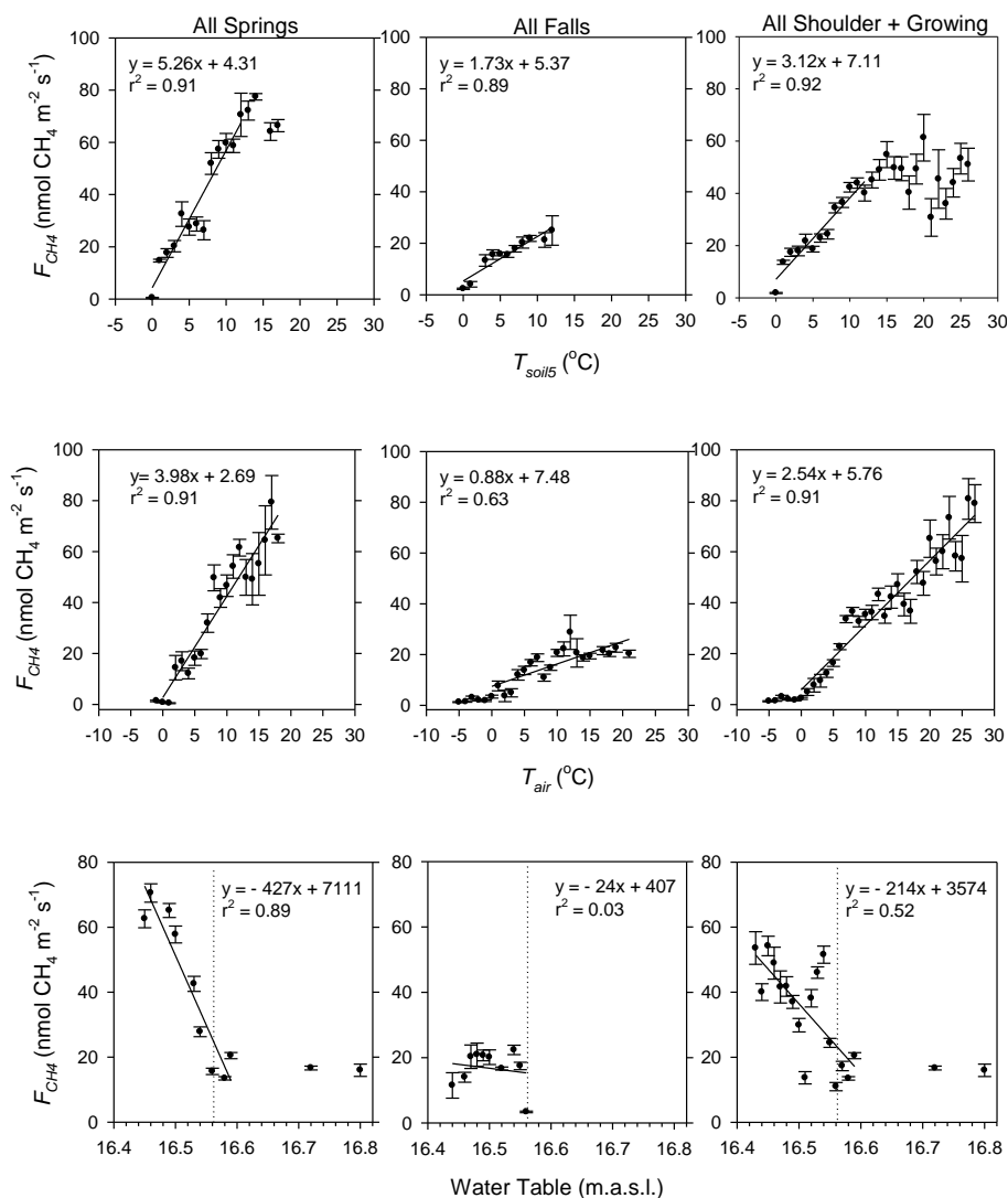
Fig. 5. Bin-averaged ( 1^{\circ}C ) 30 min F_{CH_4} \pm 1 SE in response to T_{soil5} and T_{air} shown for all springs (DOY 150 to 190, 2008–2011), all falls (DOY 260 to 320, 2008–2011) and all shoulder + growing seasons (DOY 150–320, 2008–2011). Bin-averaged (1 cm water table height) 30 min F_{CH_4} \pm 1 SE in response to water table is shown for the same periods. Dotted line indicates the mean peat surface elevation.
