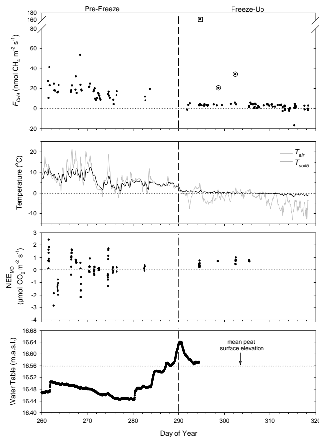
Fig. 3. Fall of 2011 30 min F_{\text{CH}_4} , T_{\text{air}} , T_{\text{soil}5} , \text{NEE}_{\text{MD}} and water table height for the fen from 17 September to 16 November 2011 (DOY 260–320). Open square indicates an anthropogenic emission burst, while open circles indicate natural emission bursts.
