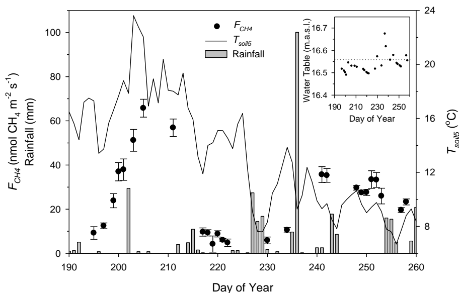
Fig. 4. Growing season mean daily F_{\text{CH}_4} (no gap-filling) ( n = 3 to 42) \pm 1 SE shown, mean daily T_{\text{soil}5} and total daily rainfall for the fen from 9 July to 17 September 2010 (DOY 190–260). Inset Figure: mean daily water table height for the fen 14 from 9 July to 17 September 2010 (DOY 190–260). Dotted line indicates the mean peat surface elevation.
