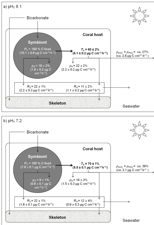
Fig. 5. Mass-balanced results of photosynthate translocation and carbon budget in Stylophora pistillata under (a) pH T 8.1, and (b) pH T 7.2 based on 13 C experiments after 48 h. Symbols are defined in the text and summarized in Table 2. Data are means ± standard error of means of n = 3 measurements.
