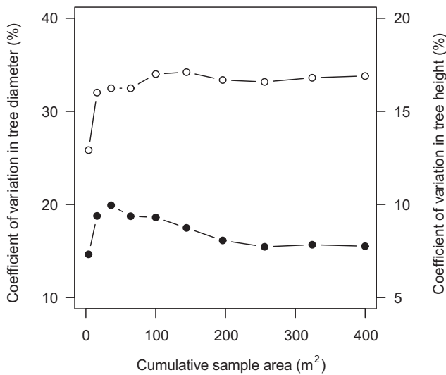
Fig. 3. Relationships of coefficient of variation of tree diameter and height to cumulative sample area in the Kandelia obovata sample plot (○ diameter, ● height).
