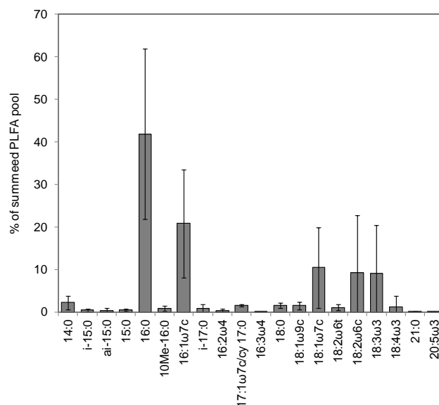
Fig. 4. Relative contributions (%) of individual PLFAs to ^{13}\text{C} -fixation in total PLFAs inhibited by nitrapyrin. Values are averages for the whole sampling period, error bars indicate corresponding standard deviations.
