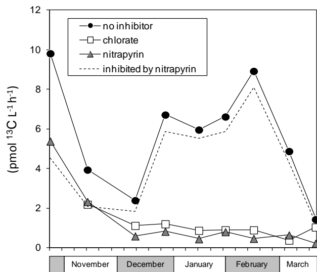
Fig. 3. Rates for ^{13}\text{C} -incorporation into summed PLFAs in incubations with nitrapyrin, chlorate, and without inhibitors. Dashed line indicates ^{13}\text{C} -fixation inhibited by nitrapyrin (difference between no inhibitor and nitrapyrin).
