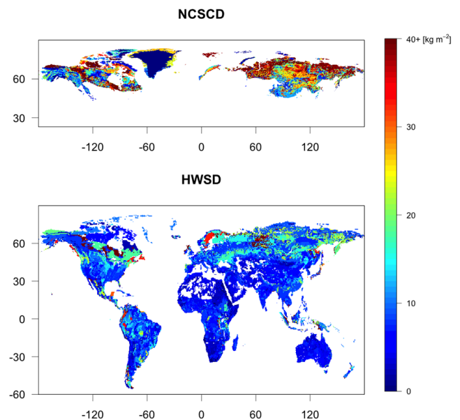
Fig. 1. Carbon density [ \text{kg m}^{-2} ] in the top 1 m of soil from the Northern Circumpolar Soil Carbon Database (NCSCD) (Tarnocai et al., 2009) and Harmonized World Soil Database (HWSD) (FAO/IIASA/ISRIC/ISSCAS/JRC, 2012).
