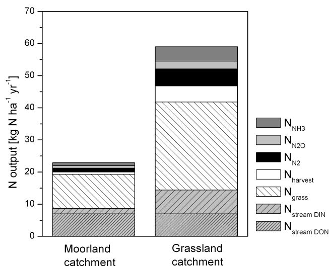
Fig. 4. N outputs ( \text{kg N ha}^{-1} \text{yr}^{-1} ) to the Moorland (left) and the Grassland catchment (right). Stream TDN export fluxes ( N_{stream} ) are split into the dissolved inorganic flux ( N_{stream\ DIN} = fluxes of \text{NH}_4^+ and \text{NO}_3^- ) and the dissolved organic flux ( N_{stream\ DON} ).
