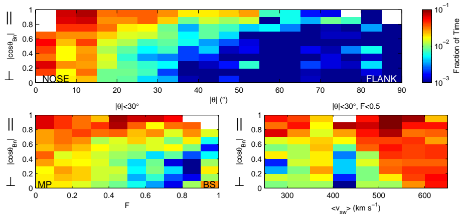
Fig. 2. Bivariate histograms where the logarithmic colour scale represents the fraction of the time that dynamic pressure enhancements ( \delta P_{\text{dyn}}/P_{\text{dyn}} > 1 ) are observed. All panels show the absolute cosine of the magnetic field – shock normal angle |\cos \theta_{Bn}| along the vertical. Across the horizontal (top) are the aberrated solar zenith angle |\theta| ; bottom left: magnetosheath fractional distance F shown for the subsolar ( |\theta| < 30^\circ ) case; and bottom right: solar wind speed for the subsolar inner ( |\theta| < 30^\circ and F < 0.5 ) magnetosheath. White areas indicate poor coverage from the magnetosheath survey.
