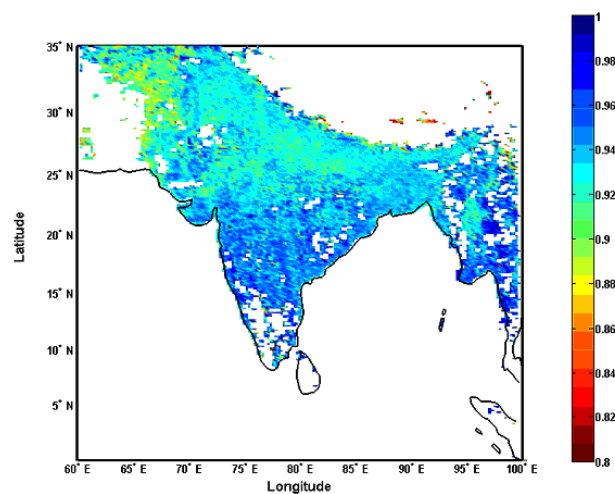
Fig. 4. Regional distribution of aerosol SSA.
