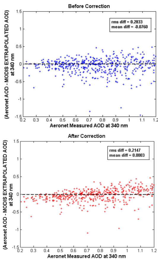
Fig. 3. The \Delta\tau_{340} versus AERONET-measured AOD at 340 nm (a) before correction, and (b) after correction.
