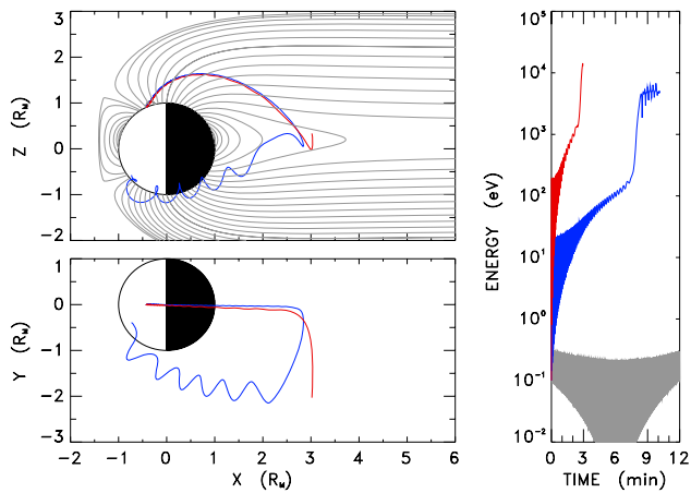
Fig. 2. Model Na + trajectories: (Left) projections in the noon-midnight meridian plane (top) and in the equatorial plane (bottom), (right) kinetic energy versus time. The test ions are launched from 65° latitude with 0.1 eV energy on the noon meridian. Three distinct cross-polar cap potential drops are considered: 1 kV, 10 kV, and 30 kV (coded in grey, blue, and red, respectively).
