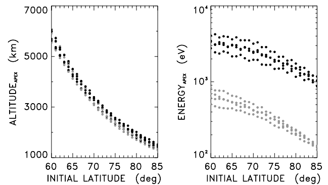
Fig. 4. Altitudes and energies obtained at \text{Na}^+ trajectory apexes as a function of initial latitude. The values obtained for \Delta\Phi = 10 kV and \Delta\Phi = 30 kV are coded in grey and black, respectively. Distinct current sheet parameters are also considered (see text).
