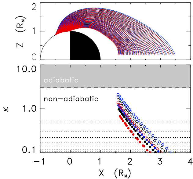
Fig. 6. (Top) Model trajectories (until apex) of \text{Na}^+ (black), \text{O}^+ (blue) and \text{Ca}^+ (red) in the noon-midnight meridian plane. (Bottom) \kappa parameter of the ions at trajectory apex versus distance X . Open and closed circles in the bottom panel show the results obtained for \Delta\Phi = 10\text{ kV} and \Delta\Phi = 30\text{ kV} , respectively. Dotted lines in this panel show the \kappa values for preferentially transient (Speiser-type) orbits.
