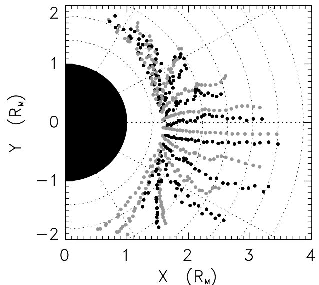
Fig. 5. \text{Na}^+ trajectory apex in the X - Y plane for different initial longitudes and latitudes in the dayside sector. The apexes obtained for \Delta\Phi = 10 kV and \Delta\Phi = 30 kV are coded in grey and black, respectively. Dotted lines show longitudes and altitudes by steps of 1000 km.
