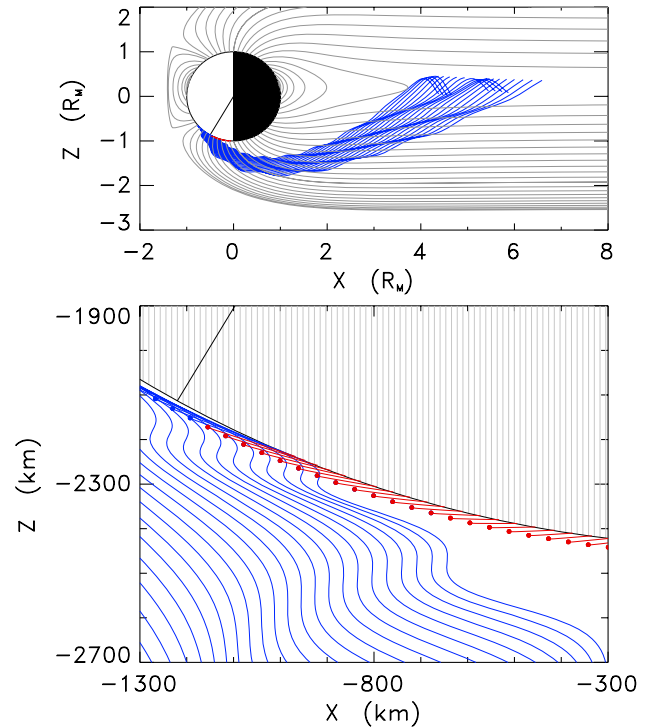
Fig. 7. Model trajectories of \text{Na}^+ ions ejected from the southern dayside sector. The bottom panel shows an enlarged view of the \text{Na}^+ paths at low altitudes. Ions that do not gain access to the magnetotail are coded in red. The solid line in both panels depicts the -60^\circ latitude.
