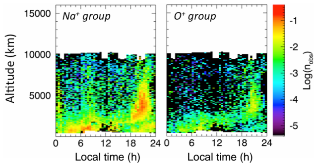
Fig. 1. Observed densities of \text{Na}^+ -group and \text{O}^+ -group ions as measured by the FIPS instrument on board MESSENGER. Densities are shown as a function of local time and altitude, and coded according to the color scale at right (adapted from Raines et al., 2013).
