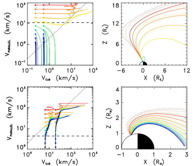
Fig. 3. (Left) Parallel speed of (top) O + ions at Earth and (bottom) Na + ions at Mercury as a function of \mathbf{E} \times \mathbf{B} drift speed. (Right) Corresponding trajectories in the noon-midnight meridian plane. The test ions are launched into the magnetosphere with different (color-coded) initial speeds. Two distinct cross-polar cap potential drops ( \Delta\Phi ) are considered: (top) 60 kV and 120 kV, (bottom) 10 kV and 30 kV. Closed circles in the left panels show the initial parallel ion speeds and \mathbf{E} \times \mathbf{B} drift speeds (of \sim 250 m s -1 and \sim 500 m s -1 at Earth, and \sim 6.5 km s -1 and \sim 20 km s -1 at Mercury). Dotted lines in the right panels show the ion trajectories achieved with the lower of the two \Delta\Phi .
