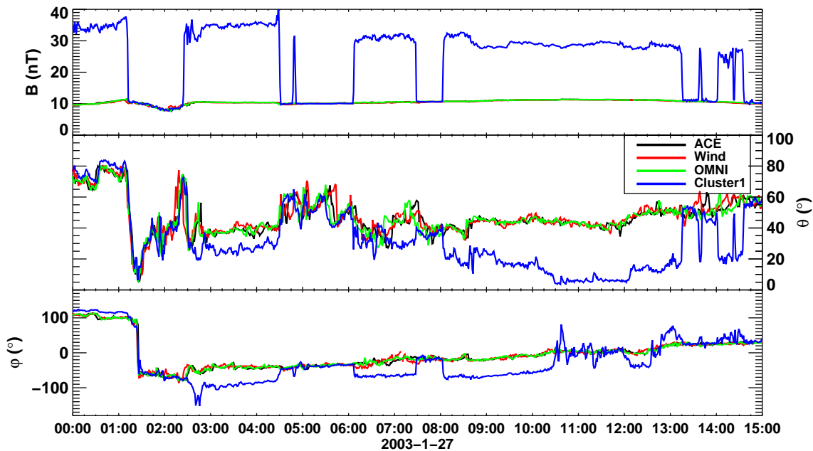
Fig. 2. Magnetic field amplitude and direction during the 27 January 2003 MC from ACE (black), Wind (red), OMNI (green) and Cluster 1 (blue) data sets – see text for definition of \theta and \phi .
