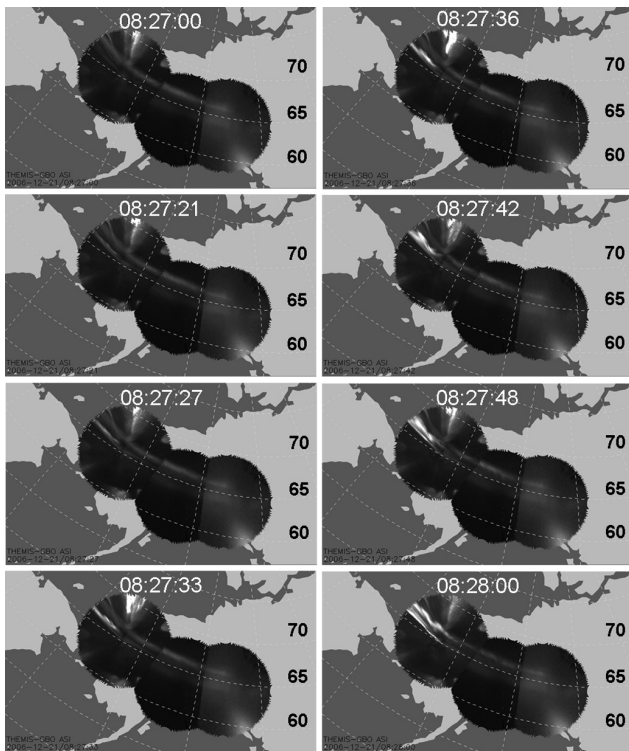
Fig. 2a. Evolution during 08:27:00–08:28:00 UT of the 21 December 2006 auroral substorm event observed by the THEMIS ground-based All-Sky-Imagers located at KIAN, GAKO, and WHIT.
