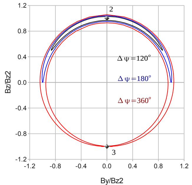
Fig. 1. Hodogram traces for A_{x2}^2 = 1.001 , \beta_2 = 1 , \gamma = 2 , and \sin^2\theta_2 = 0.996 and with three values of the net rotation angle, \Delta\Psi = 2\Psi^* , of the tangential field. Fixed Point 2 (a “center”) is at the center of the nest of traces ( B_y/B_{z2} = 0 ; B_z/B_{z2} = 1 ); Fixed Point 3 (a saddle point) is on the negative B_z -axis, at the bottom of the plot, where the red curves intersect. (From Sonnerup et al., 2010).
