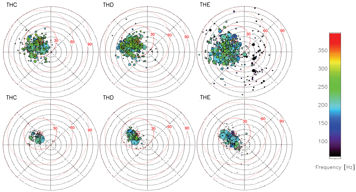
Fig. 3. Dependence of the k directions (top) and Poynting vector directions (bottom) on the frequency in GSE coordinates. Wave amplitude is coded with circle size. The direction of the local magnetic field is shown with a red cross.
