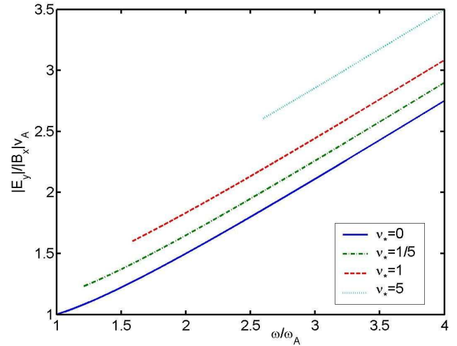
Fig. 2. The wave impedance normalized to the wave frequency. Other parameters are the same as in Fig. 1.
