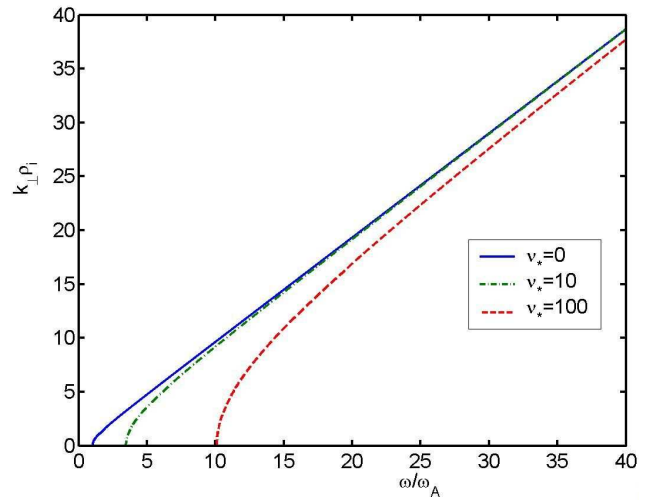
Fig. 4. The dependence of the perpendicular wave number normalized to the ion Larmor radius as a function of the normalized frequency. Calculations are carried out for the electron to ion temperature ratio T_i/T_e=14 . Solid, dash-dot, dashed lines correspond to \nu^*=0, 10 , and 100 , respectively.
