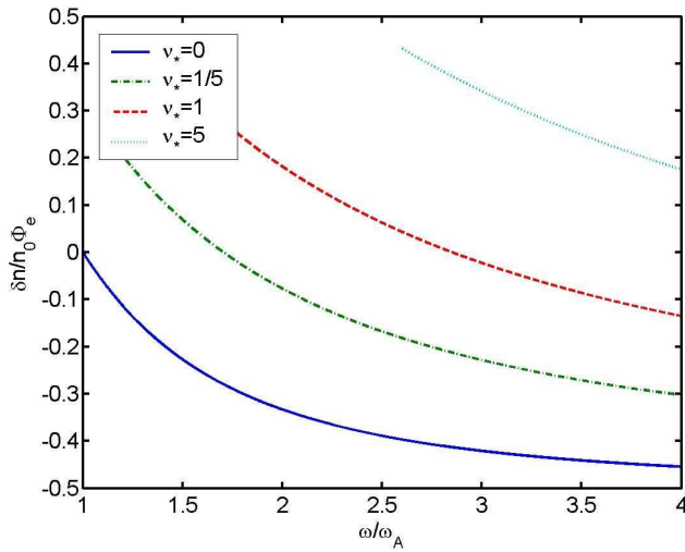
Fig. 3. The particle number density perturbations as the function of the wave frequency. Other parameters are the same as in Fig. 1.
