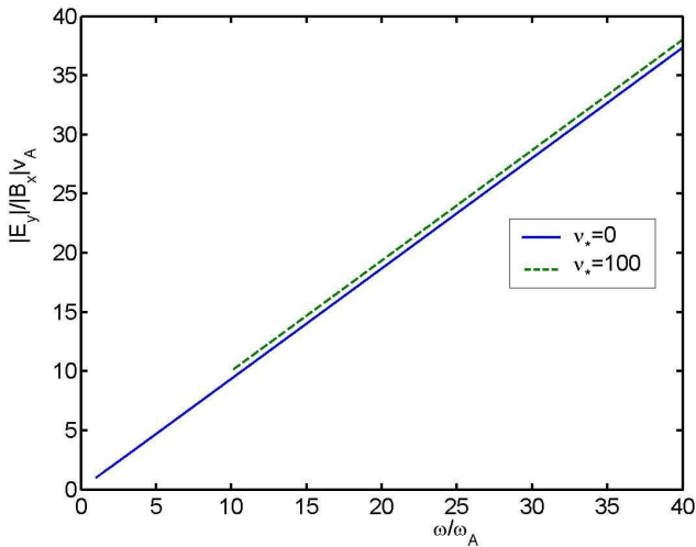
Fig. 5. The wave impedance as a function of the wave frequency. The parameters are the same as in Fig. 4.
