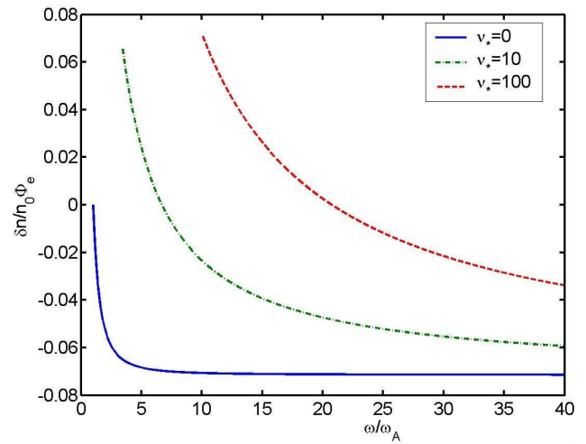
Fig. 6. Same as Fig. 5 but for the particle number density variations.
