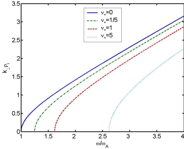
Fig. 1. The dependence of the perpendicular wave number normalized on the ion Larmor radius upon the wave frequency normalized to the Alfvén frequency. Calculations are carried out for the electron to ion temperature ratio T_e/T_i=0.5 . Solid, dash-dotted, dashed and dotted lines correspond to v_* = 0; 1/5; 1; \text{ and } 5 , respectively. With the increase of the plasma inhomogeneity (corresponding to the increase of v_* ) the wave frequency increases.
