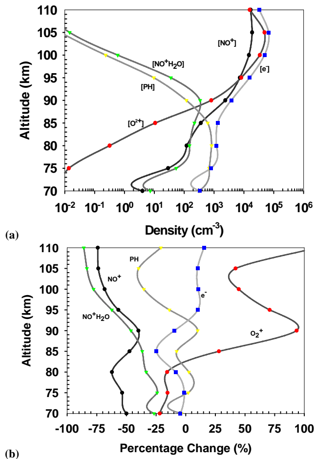
Fig. 2. (a) The number density (/cc) of major positive ions in the MLT region for background case; (b) Model results of percentage change in major positive ions for the double- \text{CO}_2 scenario in the MLT region at 10^\circ N latitude as obtained in this work.
