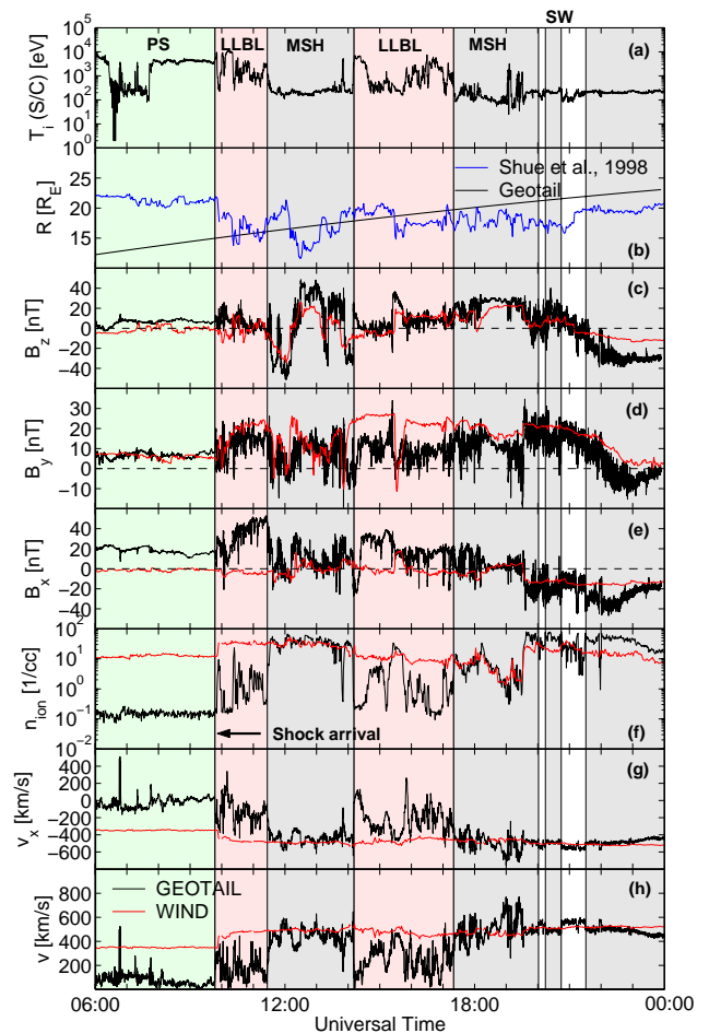
Fig. 4. Overview of Wind (red lines) and Geotail (black lines) measurements on 22 November 1997. The Wind data is propagated with 40 min and the Geotail observations are delayed by 6 min to correspond to the Polar UVI observations. From top to bottom, the figure shows the ion temperature in spacecraft coordinates T_i (in eV); the radial location of Geotail from the x-axis and the radial dimension of the magnetopause (in R_E ) predicted by Shue et al. (1998) model (blue line); the magnetic field B_z , B_y , and B_x GSM components (in nT); the ion density (in /cc); the GSM x-component of the velocity (in km/s); and the total ion bulk speed (in km/s). The different regions of the magnetosphere are shaded in different colours, light green for the Plasmasheet (PS), pink for the Low-Latitude Boundary Layer (LLBL), grey for the Magnetosheath (MSH), and white for the Solar Wind (SW). The arrival of the ICME shock is marked by an arrow.
