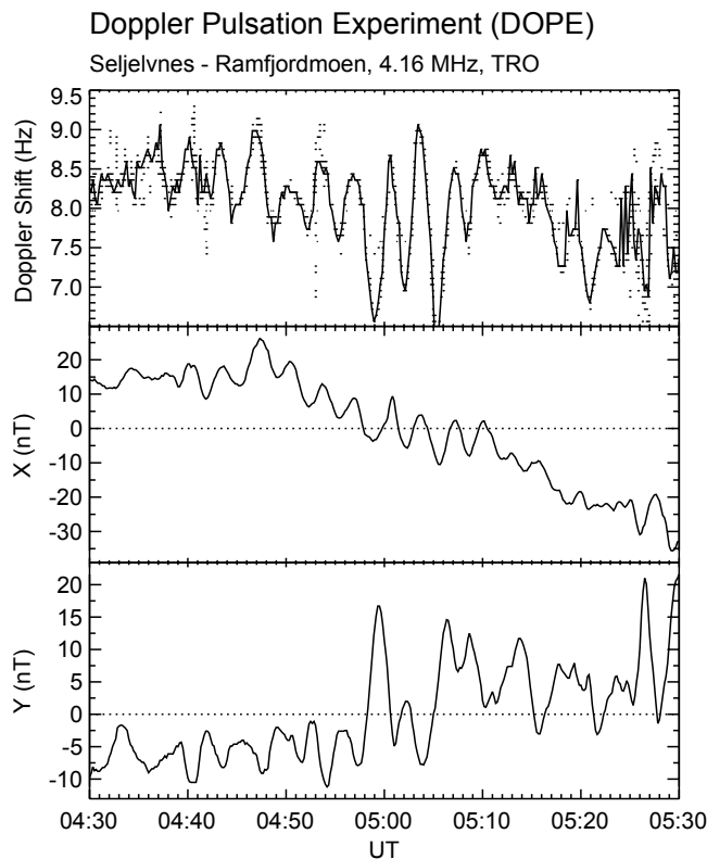
Fig. 4. DOPE and Tromsø magnetometer time series for 04:30–05:30 UT, 24 March 2001.
