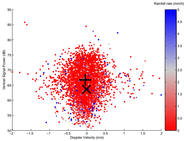
Fig. 2. Scatter plot of the variation of mean Doppler velocity and mean vertical signal power obtained using the VHF radar for the 68 days examined. Individual points are colour coded with the value of the surface rainfall rate measured by an ARG tipping bucket rain gauge. The centre of mass for the precipitation and no precipitation periods are identified by a plus sign and a cross, respectively.
