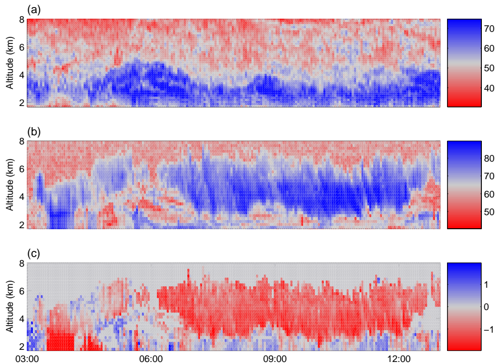
Fig. 5. Time-height contour plots of (a) vertical signal power (dB) observed by VHF radar, (b) the vertical range squared corrected signal to noise ratio (dB) and (c) the vertical velocity ( \text{ms}^{-1} ) measured by a co-located UHF wind profiler observed on 24 September 2000. Note that the UHF data has a higher time resolution than that available in the rest of this study.
