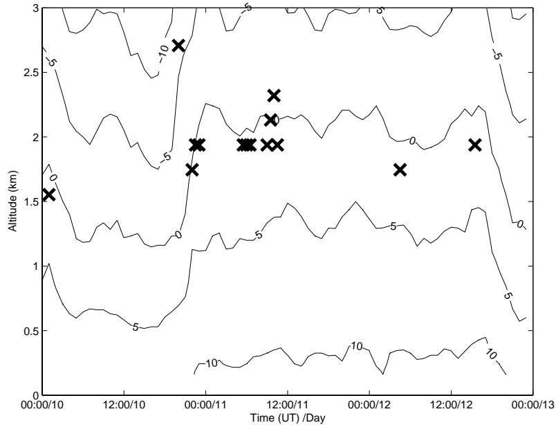
Fig. 4. Time-height contour plot of temperature taken from the UK Met Office mesoscale model predictions over Aberystwyth for the period 10 to 12 December 2000. Also displayed are crosses which indicate the position of the peak of the bright band identified by the bright band detection algorithm during this period.
