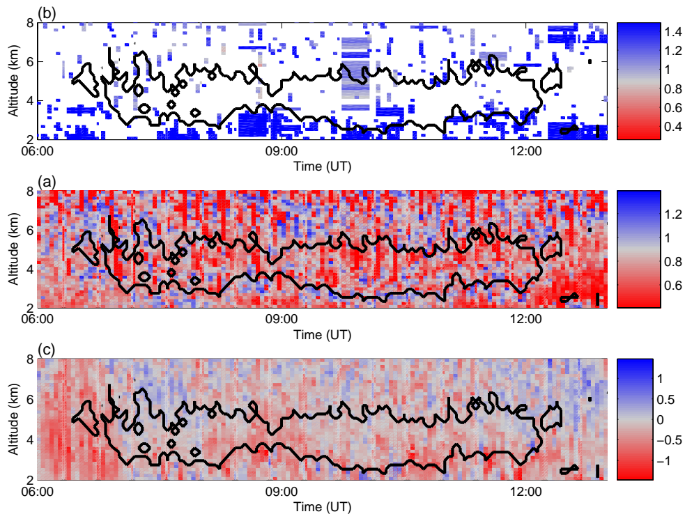
Fig. 8. Profiles of (a) precipitation signal spectral width ( \text{ms}^{-1} ), (b) clear-air signal spectral width ( \text{ms}^{-1} ), and (c) clear-air vertical velocity ( \text{ms}^{-1} ) observed by the VHF wind profiler on 24 September 2000. The full line indicates the extent of precipitating cloud regions identified using simultaneous UHF wind profiler data.
