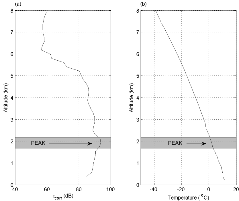
Fig. 3. Typical profiles of (a) range squared corrected signal to noise ratio, \tau_{\text{corr}} , observed by the UKMO UHF wind profiler at Aberystwyth and (b) a near simultaneous radiosonde temperature profile launched from Aberporth (approximately 50 km away from the radar site) are displayed for the 11 December 2000 at 05:30 UT. The position of the peak of the bright band identified by the automated algorithm is also displayed.
