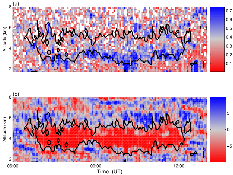
Fig. 7. Profiles of (a) vertical spectral width ( \text{ms}^{-1} ) and (b) vertical signal power perturbation (dB) observed by the VHF wind profiler on 24 September 2000. The full line indicates the extent of precipitating cloud regions identified using simultaneous UHF wind profiler data.
