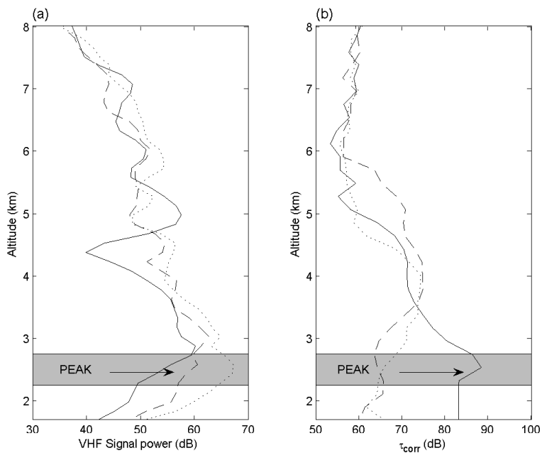
Fig. 6. Profiles of (a) vertical signal power (dB) observed by VHF radar and (b) the vertical range squared corrected signal to noise ratio (dB) measured by a co-located UHF wind profiler on 24 September 2000. The dotted line indicates the profile for 03:20 UT (outside a period of surface precipitation), the full line the profile for 03:45 UT (inside a period of surface precipitation) and the dashed line the profiles for 04:20 UT (outside a period of surface precipitation). Also displayed is a shaded region which indicates the position of the peak of the bright band identified by the Bright band detection algorithm during this period.
