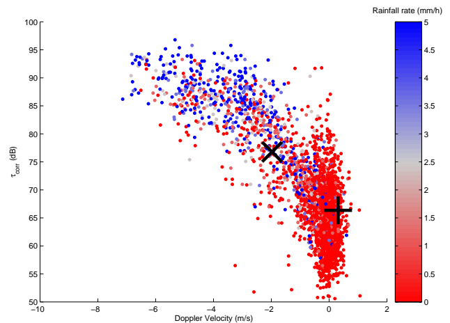
Fig. 1. Scatter plot of the variation of mean Doppler velocity and mean range squared corrected signal to noise ratio, \tau_{\text{corr}} , obtained from the vertical beam of the UKMO UHF wind-profiler for the 68 days examined. Individual points are colour coded with the value of the surface rainfall rate measured by an ARG tipping bucket rain gauge. The centre of mass for the precipitation and no precipitation periods are identified by a plus sign and a cross, respectively.
