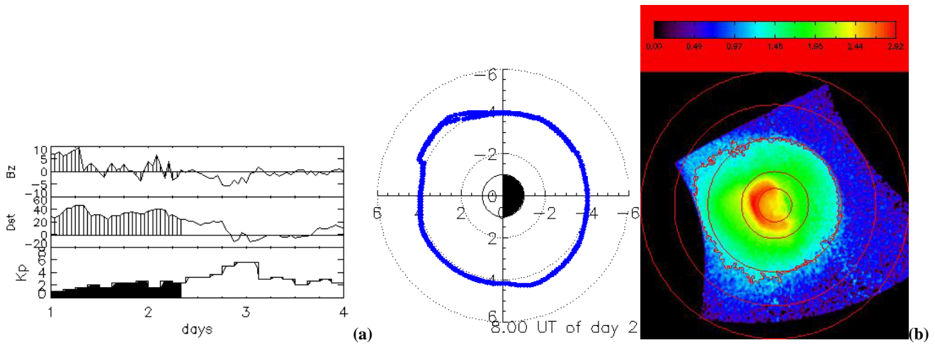
Fig. 1. (a) Result of the simulation based on the instability mechanism, the ESD model and the value of K_p on 9 June 2001, 08:00. The plasmapause in the geomagnetic equatorial plane corresponds to the blue line. The indexes B_z , D_{st} and K_p , observed during the previous and following days, are also displayed. The dotted circles correspond to L=1, 2, 4 and 6 . (b) EUV observations on 9 June 2001 at 08:00 UT, projected in the geomagnetic equatorial plane. The red line corresponds to 40% of the maximum intensity of the image and permits one to visualize the plasmapause. The red circles correspond to L=1, 2, 4, 6 and 8 .
