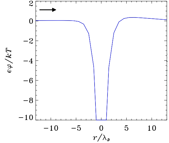
Fig. 3. Potential distribution along the x -axis parallel to the bulk velocity in an O + plasma with V_0=4V_{Ti} . Plasma parameters and probe potential are the same as in Fig. 2, where the potential is normalized by plasma temperature. Direction of the bulk velocity is indicated by an arrow.
