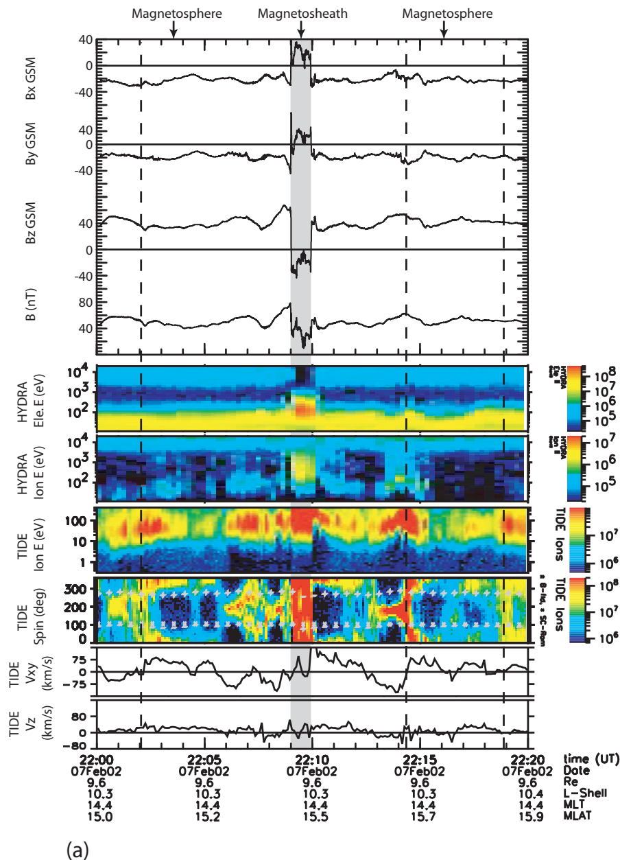
Fig. 5. Magnetopause crossings during the intervals (a) 22:00–22:20 UT and (b) 23:10–23:30 UT. Shown, from top to bottom, are the highest time resolution (8 samples/s) magnetic field data, the HYDRA ion and electron energy spectrograms, the TIDE ion energy and spin angle spectrograms, and the TIDE ion velocity moment data. The ion velocity components V_{xy} and V_z shown in the bottom panels are the spin plane velocity projected to the equatorial plane (nearly aligned to the radial direction) and along the Z-axis (north), respectively.
