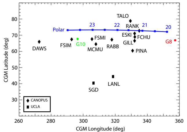
Fig. 9. The ground stations and spacecraft footprints in the North American sector in the Corrected GeoMagnetic (CGM) coordinates.
