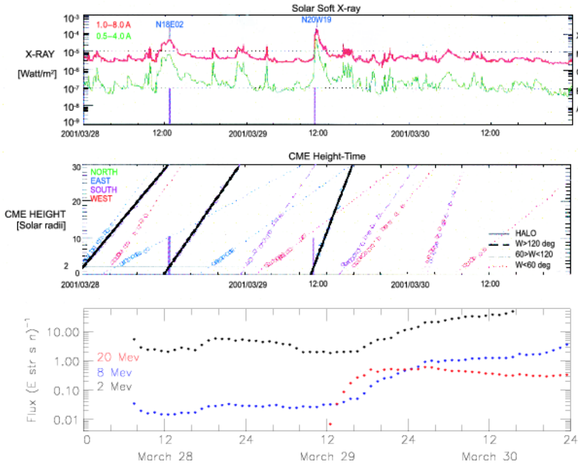
Fig. 8. Solar observations (top panels). Bottom panel: LEMT/EPACT measurements of high energy proton fluxes. A dispersal injection is seen starting at \sim 12:00 UT, 29 March in the highest energy panel.
