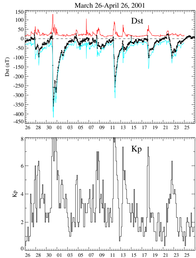
Fig. 10. K_p and D_{st} measurements for 26 March–26 April 2001. The effect of the \alpha -particles in calculating the magnetopause currents (top red trace) has not been taken into account. For further details, see text.
