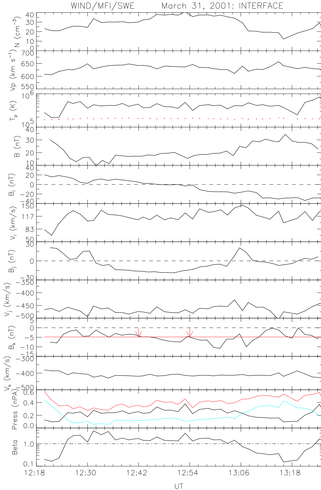
Fig. 9. The interface between ejecta 1 and 2. The panels show from top to bottom the proton density, bulk speed and temperature, (pairwise) components of field and flow in principal axes coordinates (i, j, k); the pressures (blue: magnetic field, black: plasma (electrons plus protons) and red: their sum), and the proton beta.
