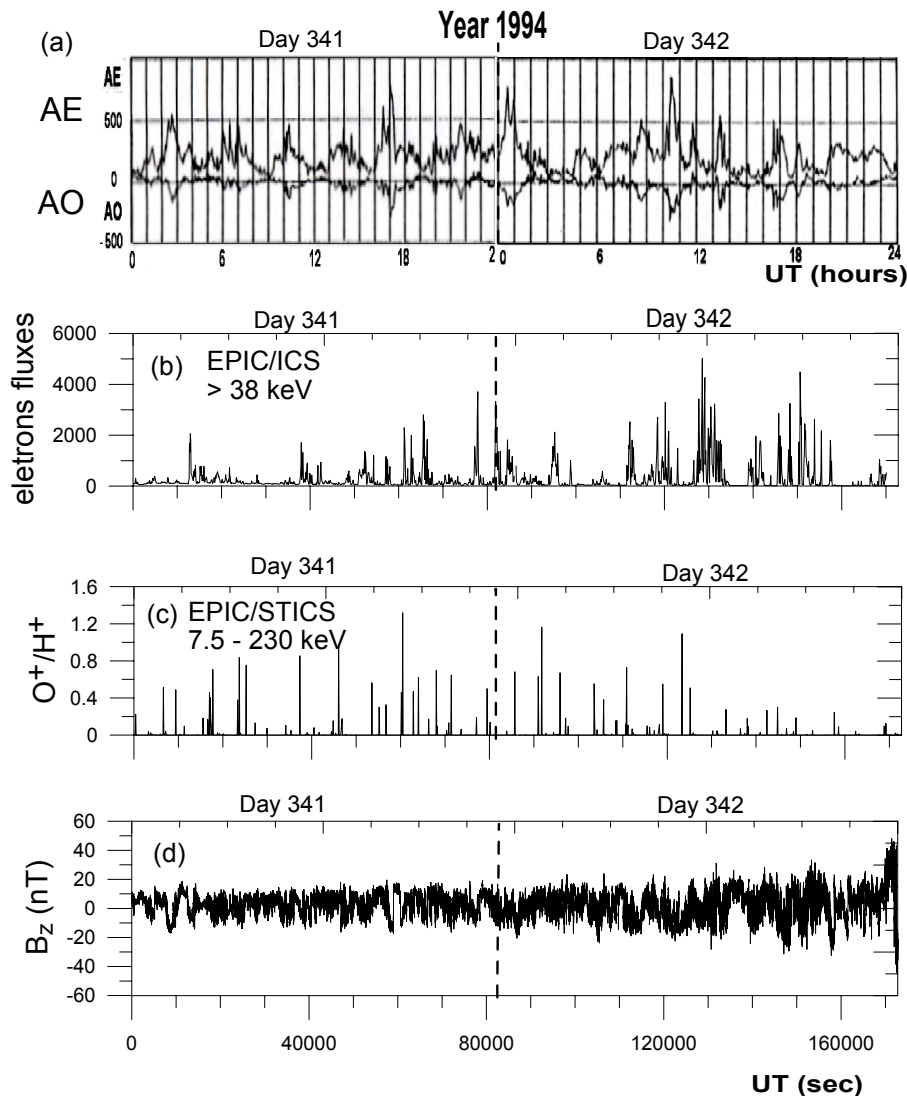
Fig. 6. From top to bottom, (a) AE index measurements with one minute resolution, (b) the energetic >38 keV electrons (second panel), (c) the ratio O^+/H^+ (third panel) and (d) the B_z component (fourth panel).
