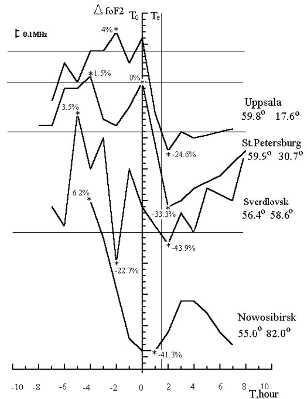
Fig. 11. The variations of \Delta foF2 values for the positive substorm that occurred on 05 March 1999 ( T_o = 16:00 UT, I = +220 nT, \tau = 1.5 h) through the latitudinal chain of stations of the IDCE, Upp.: LT = UT + 2, St. P.: LT = UT + 3, Sv.: LT = UT + 6, Now.: LT = UT + 7. The vertical lines mark substorm onset, T_o , and the end of the substorm, T_e . Asterisks are \delta foF2 (%) values.
