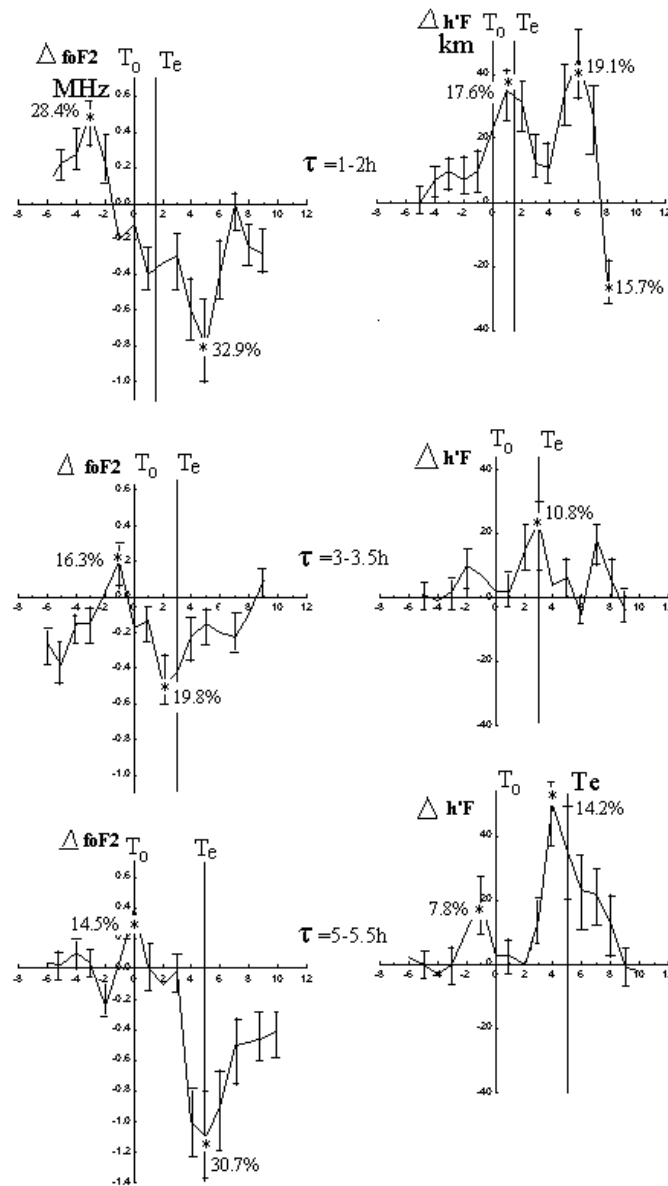
Fig. 3. The average variations of \Delta foF2 and \Delta h'F separated by duration into 3 classes: \tau = 1 - 2\text{h} , \tau = 3 - 3.5\text{h} , and \tau = 5 - 5.5\text{h} . The vertical lines mark substorm onset, T_0 and the average end of the substorm, T_e . Asterisks are \delta foF2 (%) and \delta h'F (%) values.
