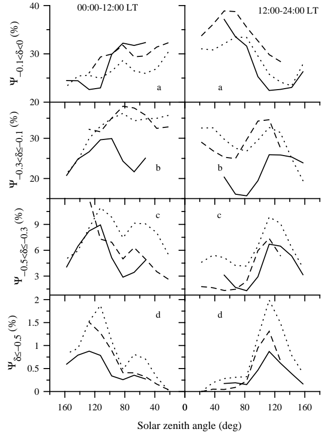
Fig. 9. The dependence of the NmF2 negative disturbance probability functions on the solar zenith angle in latitude range 4 ( 45^\circ < |\varphi| \leq 60^\circ , 45^\circ < |\Phi| \leq 60^\circ ) during the winter (solid lines), summer (dashed lines), and spring and autumn (dotted lines) months for the weak (panels a), normal (panels b), strong (panels c), and very strong (panels d) NmF2 negative disturbances. The 0^\circ - 180^\circ solar zenith angle range includes the local time period from 00:00 LT to 12:00 LT (left panels) and from 12:00 LT to 24:00 LT (right panels).
