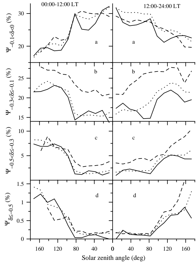
Fig. 7. The dependence of the NmF2 negative disturbance probability functions on the solar zenith angle in latitude range 2 ( 10^\circ < |\Phi| \leq 30^\circ ) during the winter (solid lines), summer (dashed lines), and spring and autumn (dotted lines) months for the weak (panels a), normal (panels b), strong (panels c), and very strong (panels d) NmF2 negative disturbances. The 0^\circ - 180^\circ solar zenith angle range includes the local time period from 00:00 LT to 12:00 LT (left panels) and from 12:00 LT to 24:00 LT (right panels).
