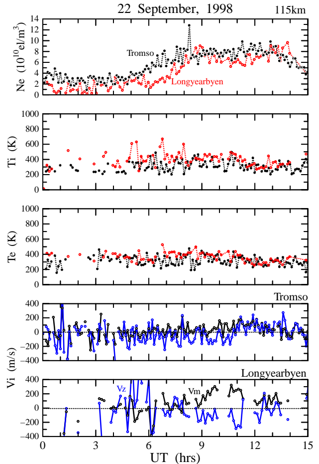
Fig. 4. Summary plots of the ionospheric parameters at 115 km altitude measured by the Tromsø radar and by the Svalbard radar from 00:00 to 15:00 UT on 22 September 1998. The top panel shows the electron density obtained from the field-aligned beam at Tromsø (black) and Longyearbyen (red). The ion and electron temperatures obtained from the field-aligned beam at Tromsø (black) and Longyearbyen (red) are shown in the second and third panels, respectively. The derived ion velocities at Tromsø and Longyearbyen are plotted in the fourth and fifth panels, respectively. The meridional component ( V_m ) is shown by the black line, and the zonal component ( V_z ) the blue line. The positive values indicate the northward and eastward components.
