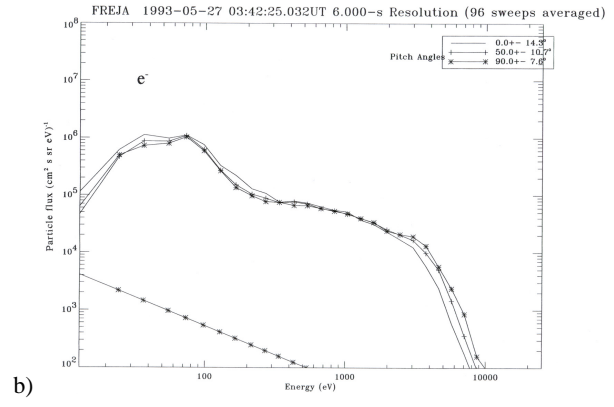
Fig. 20. Measured energy spectra of H^+ ions (count rate) (a) and energetic electrons (differential particle flux) (b) when the ion energies reached the upper energy limit of the spectrometer in Fig. 18. Straight lines show 1-count levels.
