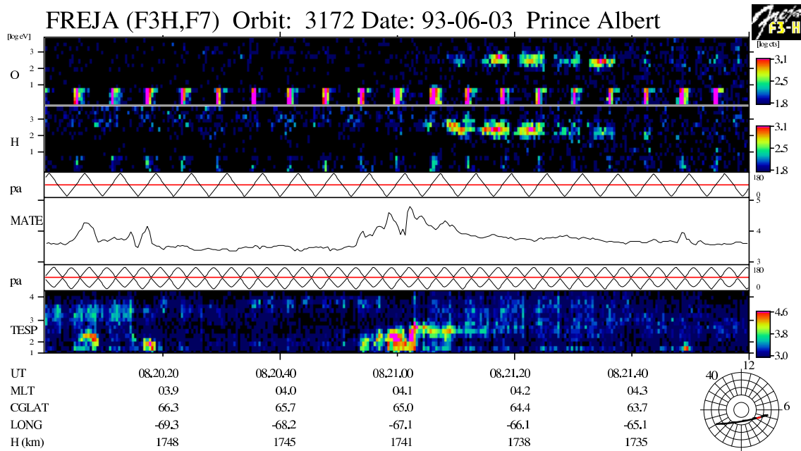
Fig. 2. A CSP of the higher time resolution type, covering 2 min of time. It shows the period of orbit 3172 in Fig. 1 when precipitating ions were recorded. This higher time resolution CSP differs from the low time resolution kind shown in Fig. 1 only in that frames 3 and 5 contain pitch-angle data instead of auxiliary information.
