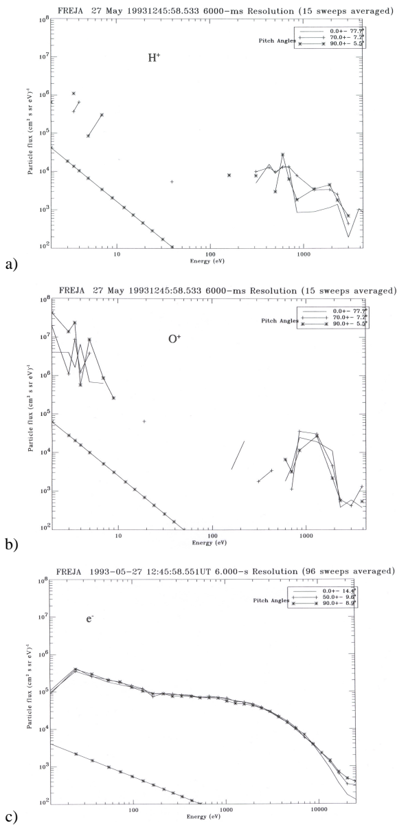
Fig. 8. Detailed energy spectra measured in orbit 3082 of precipitated H^+ ions (a) and O^+ ions (b) and of the precipitated electrons (c). Straight lines show 1-count level.
