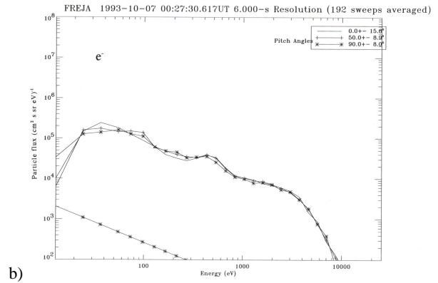
Fig. 17. Measured energy spectra of H^+ ions (a) and electrons (b) before the ion energy started to decrease in Fig. 15.
