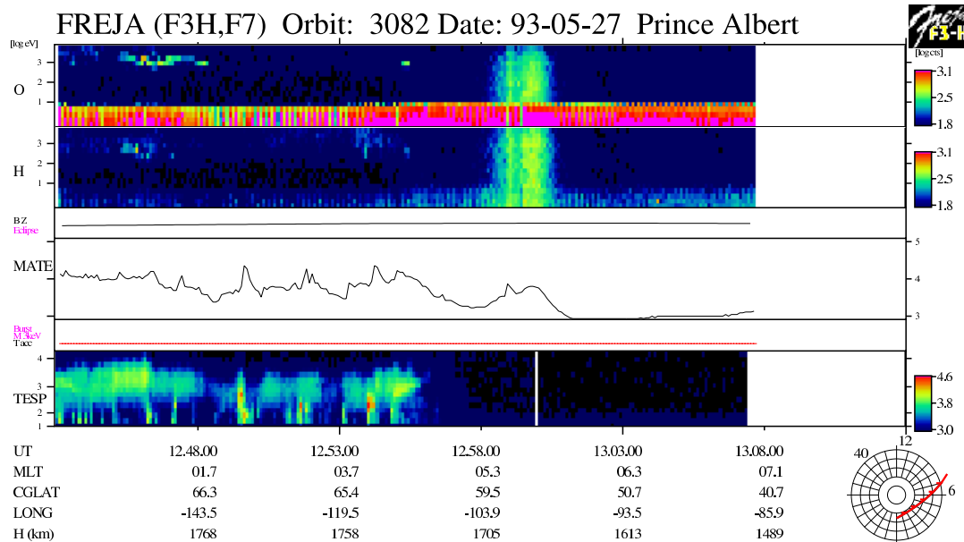
Fig. 6. A full-pass CSP for orbit 3082, covering MLT from midnight to 07:00 and CGLAT 67–42°. In the ion precipitation region there are mostly higher peak count rates of O + ions than of H + .
