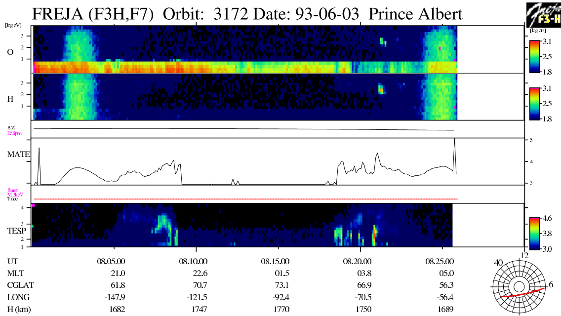
Fig. 1. Example of a Color Summary Plot (CSP) for a high-latitude pass of Freja. The satellite orbit is indicated in the circular coordinate system at the lower right (magnetic local time, MLT, and corrected geomagnetic latitude, CGLAT). The two uppermost frames show the logarithm of the count rate, color-coded as a function of time and the logarithm of the energy of O^+ and H^+ ions measured by means of the TICS spectrometer. Frames 3 and 5 may contain some auxiliary data (not used in this investigation) and frames 4 and 6 show electron data from the MATE and TESP instruments, total particle flux in the energy range from a fraction of a keV to about 100 keV in the case of MATE and the count rate, color-coded, of the electrons as a function of time and energy from TESP. UT, MLT, CGLAT, LONG (geographic) and altitude, H, are listed at the bottom. A description of the various recorded count rates and what they represent can be found in the text. The data of particular interest in the present investigation are the relatively intense ion count rates seen in a short period of half a minute at about 08:21 UT.
