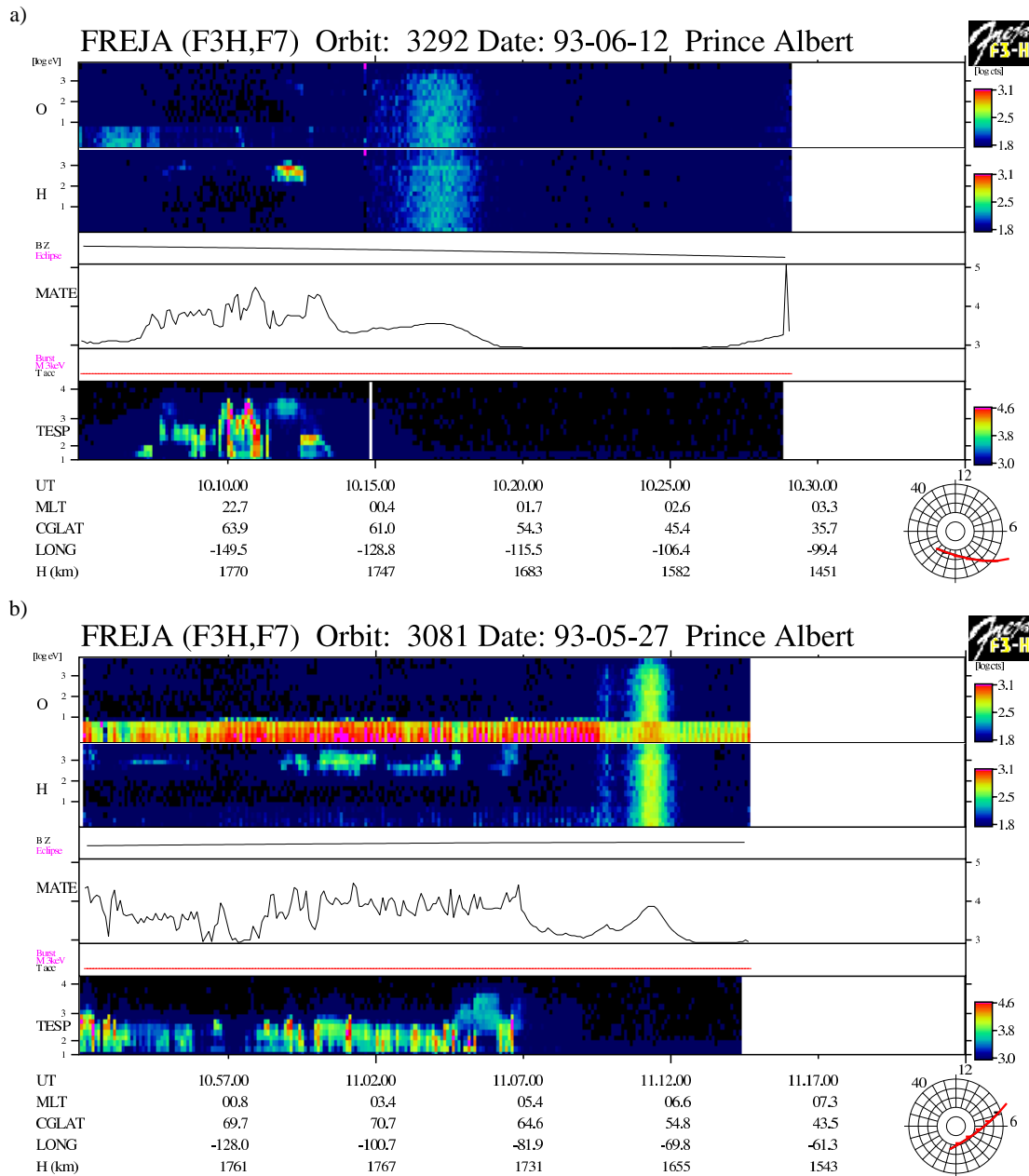
Fig. 24. Precipitating ions occur (almost only) in a period when the electron energy spectrum is like an un-accelerated typical plasma sheet spectrum in (a). In (b) the only major gap in the H + ion precipitation coincides with a period with such a plasma-sheet electron spectrum.
