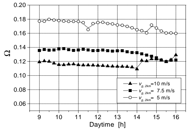
Fig. 3. Dependence of the decoupling coefficient \Omega on geostrophic wind speed; simulation with the model HIRVAC for 3 July and clear sky ( h_{veg} = 27.5 m, n_w = 0.8 , LAI = 5 ).
