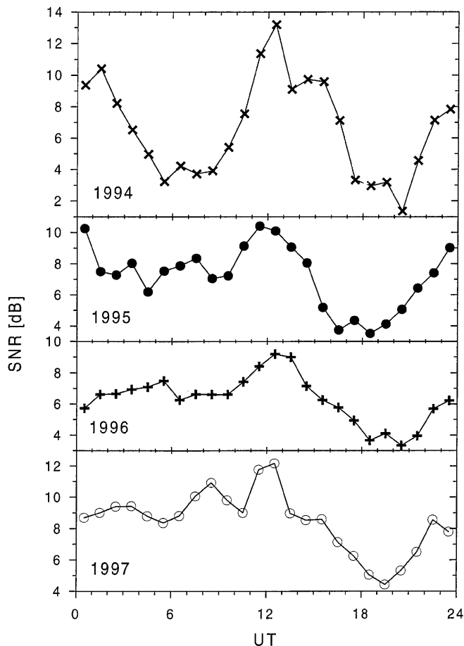
Fig. 9. Diurnal variation of SNR (83.0–87.5 km, Andenes) for the years 1994–1997 with data from June and July
