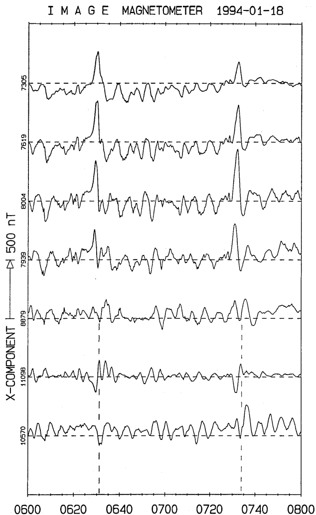
Fig. 1. Magnetograms obtained along a meridian chain from Svalbard to Scandinavia showing as an example the occurrence of two large-amplitude TCVs ( dashed lines ). The bottom trace shows the
