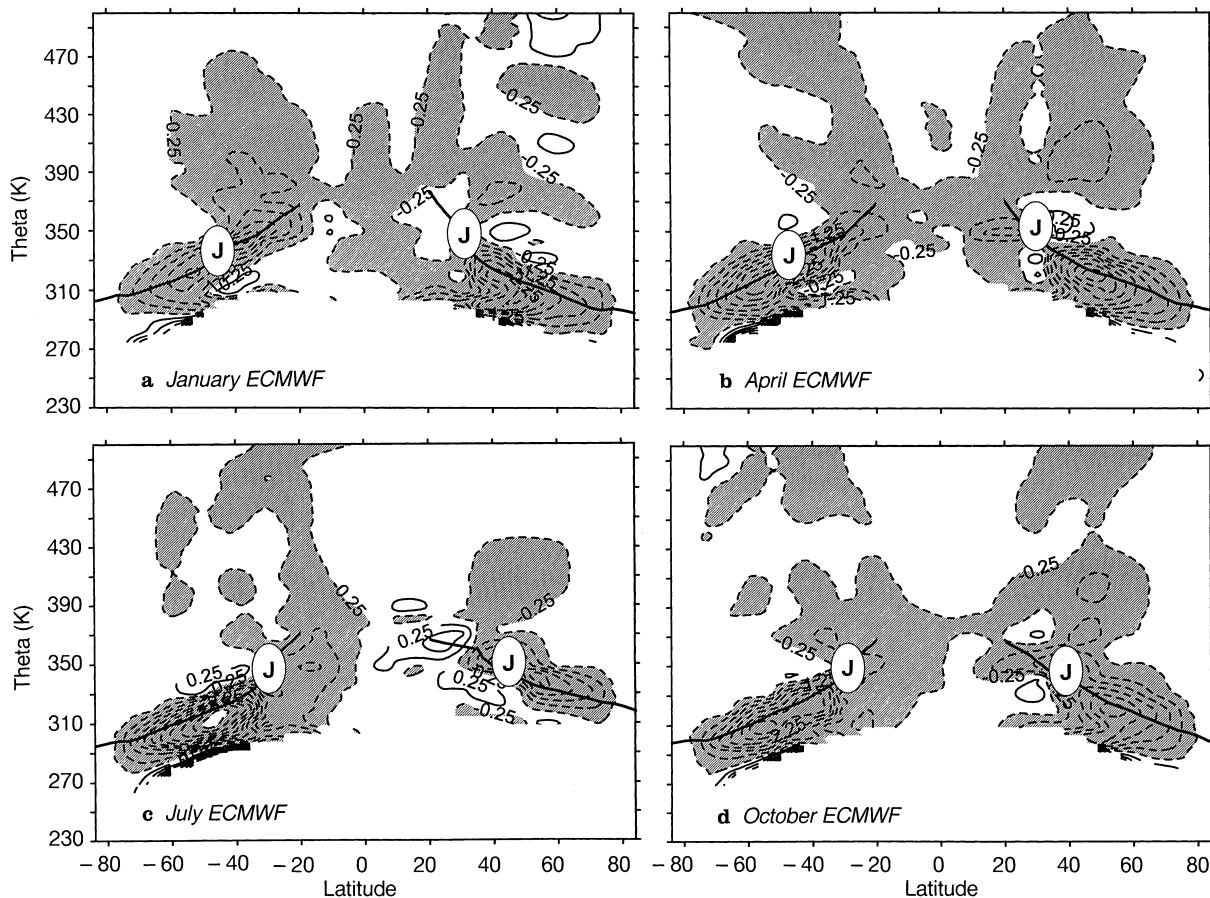
Fig. 3a–d. Zonally averaged meridional transient eddy PV flux multiplied by \cos \phi in 10^{-5} \text{ m s}^{-2} from ECMWF analysis for 4 months. The contour interval is 0.5. Negative contours are dashed.
