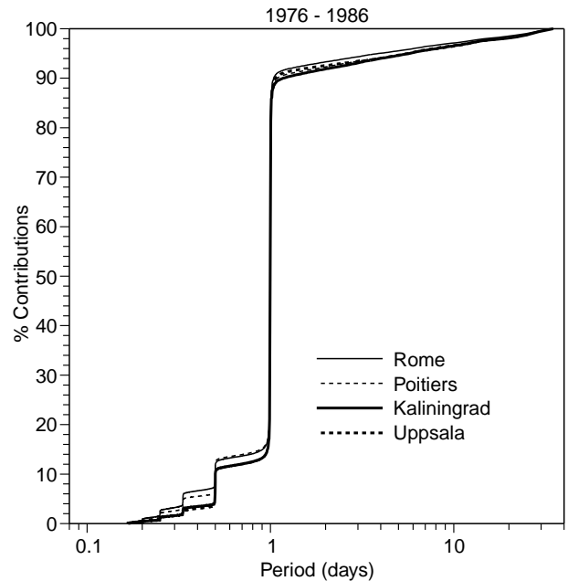
Fig. 2. Integrated percent contributions for periods lower than a given value in the periodic range from 4 h to 35 days for the whole solar cycle
