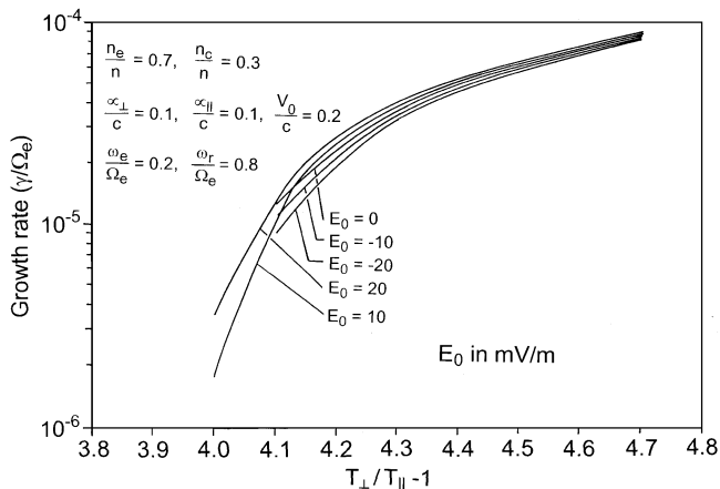
Fig. 3. Variation of growth rate ( \gamma/\Omega_e ) with (T_{\perp}/T_{\parallel} - 1) for \omega_e/\Omega_e = 0.2, \alpha_{\parallel}/c = \alpha_{\perp}/c = 0.1, v_0/c = 0.2, n_c/n_c = 0.7 , and for different values of E_0 = 0, 10, 20 mV/m
