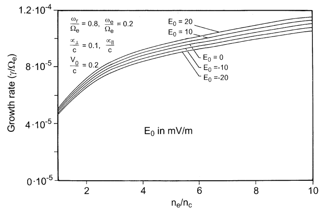
Fig. 5. Variation of growth rate ( \gamma/\Omega_e ) with n_e/n_c for \alpha_{\perp}/c = \alpha_{\parallel}/c = 0.1, v_0/c = 0.2, \omega_e/\Omega_e = 0.2 , and for different values of E_0 = 0, 10, 20 mV/m
