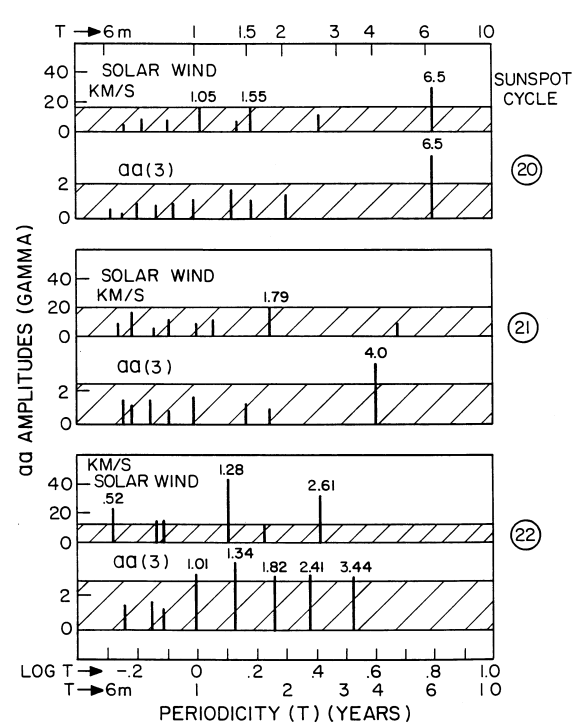
Fig. 9. Spectra for 3-monthly means of solar wind and aa indices for cycles 20, 21, 22 separately
