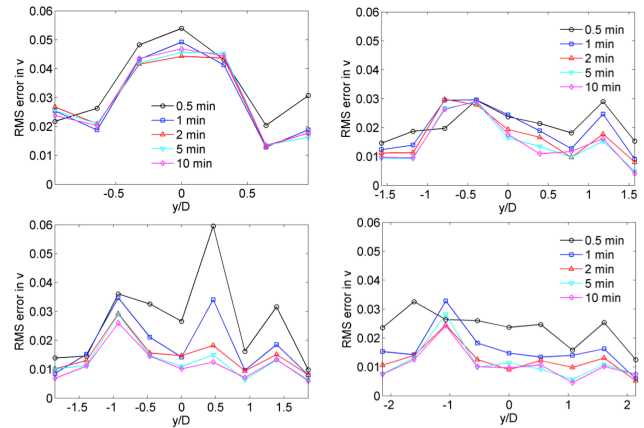
Figure 9. RMS global error (normalized by hub-height inflow wind speed U_H of 6.5 \text{ m s}^{-1} ) in the cross-stream component across the wake at different distances downstream with the lidar range weighting function applied: x/D = 3 (top left), x/D = 5 (top right), x/D = 7 (bottom left), x/D = 9 (bottom right); the different colors denote averaging times.
