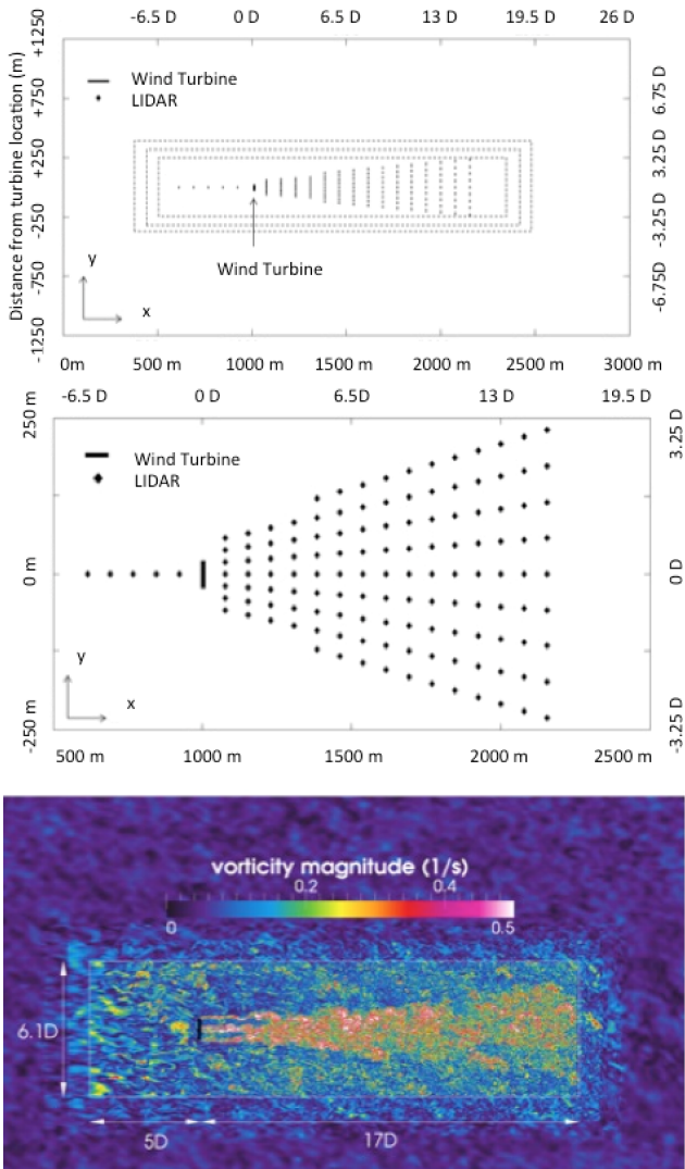
Figure 1. Simulation domain for precursor and turbine-resolving domains (top), with zoomed-in version (center) identifying lidar locations in the wake of the wind turbine and contours (bottom) of vorticity in the turbine-resolving domain. The nests (top) denote the regions with grid refinement from 10 to 5 to 2.5 to 1.25 m resolution. Flow is from west to east at the turbine hub height.
