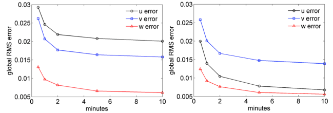
Figure 6. RMS global error (normalized by hub-height wind speed U_H of 6.5 \text{ m s}^{-1} ) at all lidar locations and all heights, normalized by the upwind hub-height wind speed, as a function of averaging time with the lidar range weighting function applied (left) and without the lidar range weighting function applied (right).
