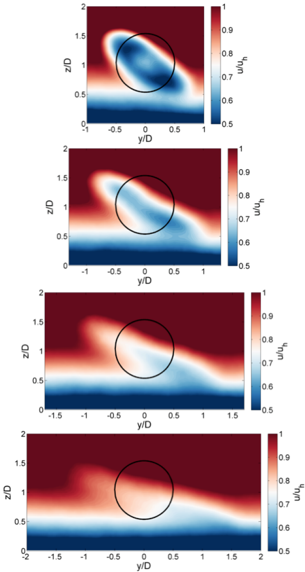
Figure 3. Cross-stream slices of stream-wise velocity, normalized by upwind hub-height wind speed ( 6.5 \text{ m s}^{-1} ) at 3 D (top), 5 D , 7 D , and 10 D (bottom) downwind of the turbine. The perspective is looking upwind. The large black circle outlines the location of the turbine rotor disk inscribed by the actuator line model.
