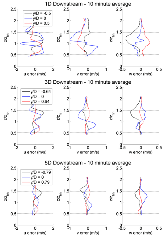
Figure 11. Profiles of error (Eq. 5) in lidar measurements of stream-wise (left), cross-stream (center), and vertical (right) wind speed, with the lidar range weighting function applied, from lidars located 1 D (top), 3 D (center), and 5 D (bottom) downwind of the turbine. Locations of the lidars are at the center and the cross-stream edges of the wakes as labeled in the figures.
