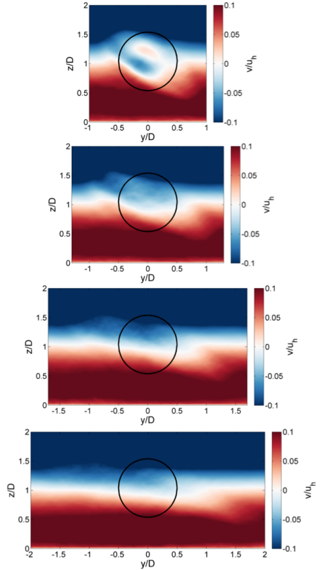
Figure 4. Cross-stream slices of cross-stream velocity, normalized by upwind hub-height wind speed ( 6.5 \text{ m s}^{-1} ) at 3 D (top), 5 D , 7 D , and 10 D (bottom) downwind of the turbine. The perspective is looking upwind. The large black circle outlines the location of the turbine rotor disk inscribed by the actuator line model.
