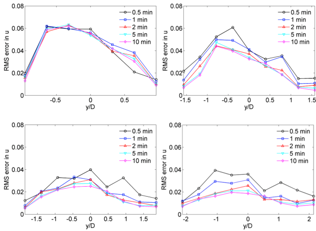
Figure 8. RMS global error (normalized by hub-height inflow wind speed U_H of 6.5 \text{ m s}^{-1} ) in the stream-wise component across the wake at different distances downstream: x/D = 3 (top left), x/D = 5 (top right), x/D = 7 (bottom left), x/D = 9 (bottom right) with the lidar range weighting function applied; the different colors denote averaging times.
