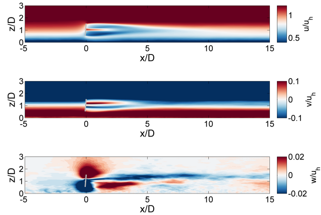
Figure 2. 10 min averaged contours of wind speed in the stream-wise (top), cross-stream (middle), and vertical (bottom) directions, normalized by average hub-height inflow wind speed ( 6.5 \text{ m s}^{-1} ), taken along the turbine location at y = 0 \text{ m} (Fig. 1) after equilibration.
