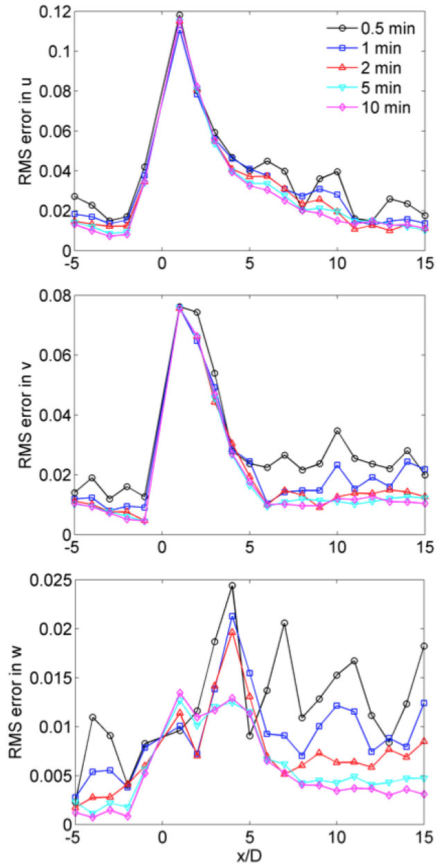
Figure 7. RMS global error (normalized by hub-height inflow wind speed U_H of 6.5 \text{ m s}^{-1} ) for each lidar situated along the turbine-wake centerline ( y = 0 \text{ m} and y/D = 0 in Fig. 1) with the lidar range weighting function applied. Stream-wise error (top), cross-stream error (middle), and vertical velocity error (bottom). Each color represents a different amount of time averaging.
