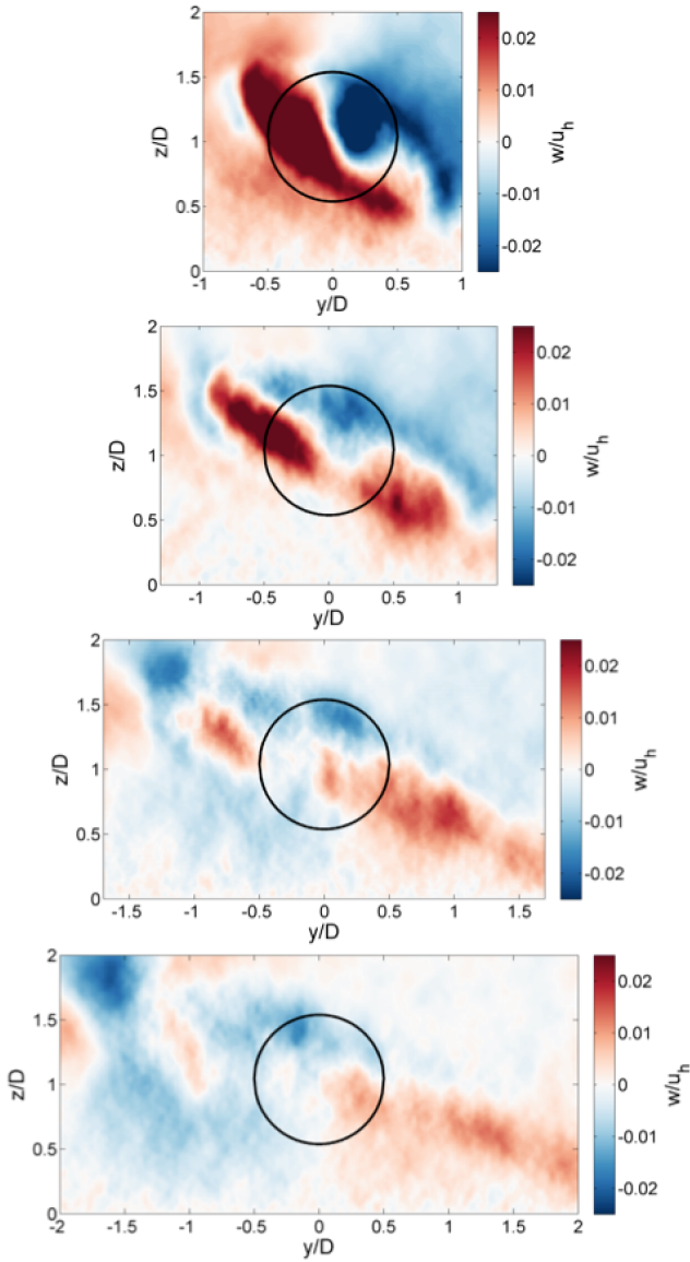
Figure 5. Cross-stream slices of vertical velocity, normalized by upwind hub-height wind speed ( 6.5 \text{ m s}^{-1} ) at 3 D (top), 5 , 7 , and 10 D (bottom) downwind of the turbine. The perspective is looking upwind. The large black circle outlines the location of the turbine rotor disk inscribed by the actuator line model.
